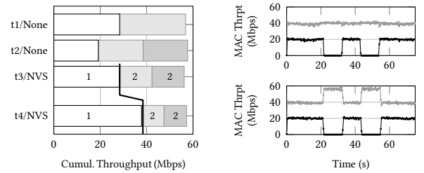
(a) Isolation (UEs are marked) (b) Static resource attribution vs. resource sharing.
