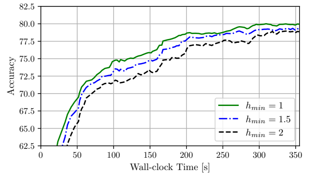
Fig. 3. Test accuracy versus time under different channel gain thresholds. Smaller thresholds result in larger average consensus rates and therefore in faster convergence.
