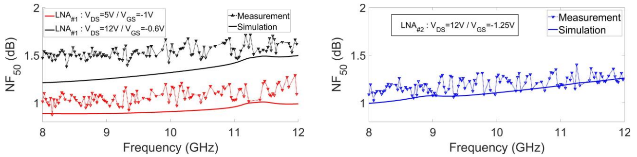
Fig. 6 : Simulated and measured X-band noise figure for LNA #1 [in its low noise configuration ( V_{DS}=5V / V_{GS}=-1V ), in EM aggression mode ( V_{DS}=12V / V_{GS}=-0.6V )] and for LNA #2 ( V_{DS}=12V / V_{GS}=-1.25V )
