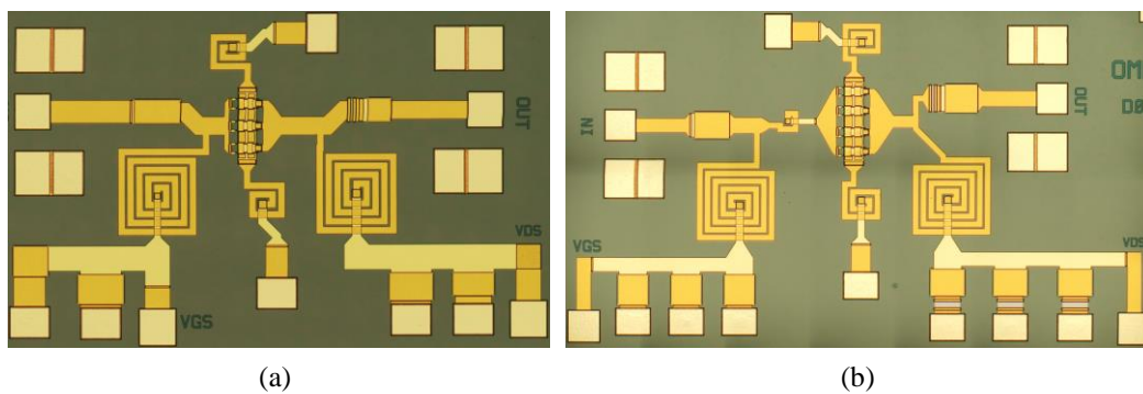
Fig. 3 : Layout of the two LNAs considered for the study: (a) LNA#1 with the 6*40\mu m transistor, (b) LNA#2 with the 8*50\mu m transistor.
