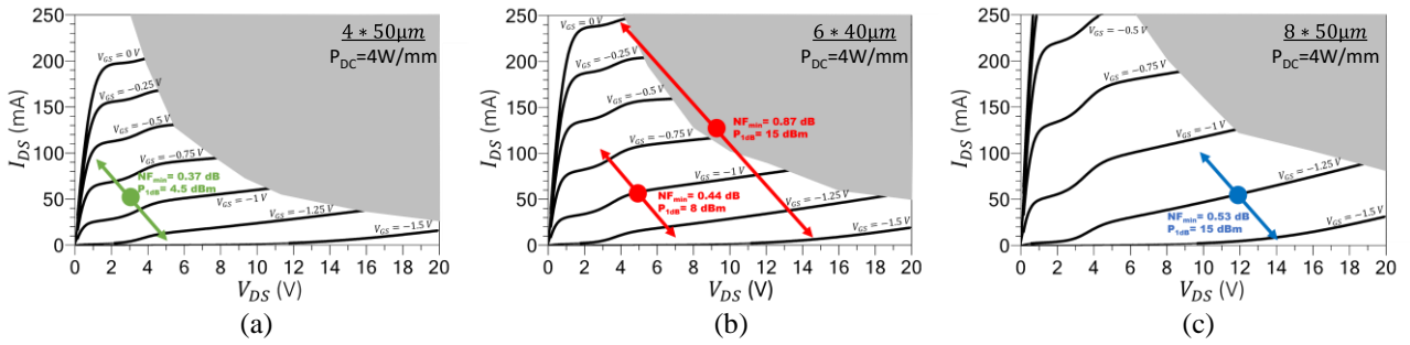
Fig. 2 : Static characteristics [ I_{DS}(V_{DS}) ] for three transistor dimensions ( 4*50\mu m , 6*40\mu m & 8*50\mu m ). Each quiescent point appears with NF_{min} and associated P_{1dB} . The areas of maximum DC power dissipation are shown in gray.
