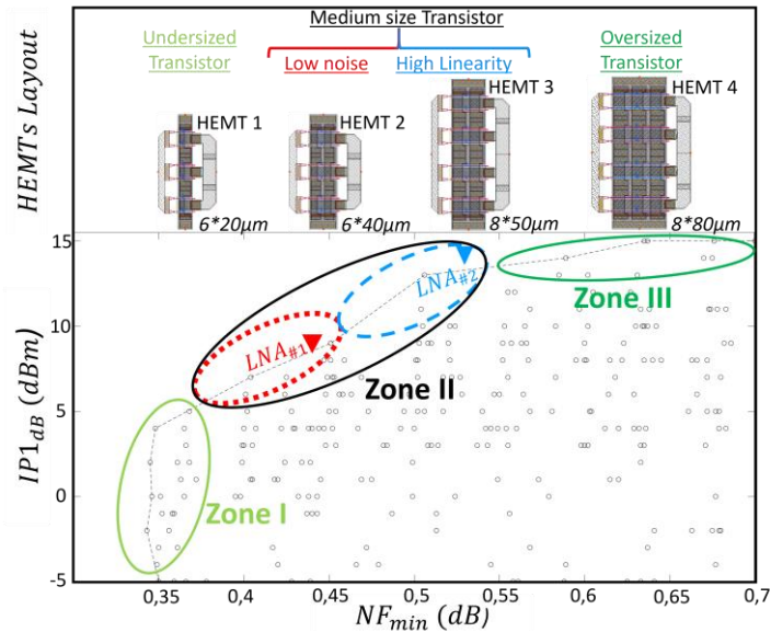
Fig. 1 : Device biasing and sizing selection for Low Noise or high compression IP1dB purposes (NFmin versus IP1dB @ 10 GHz). Sizing is for number of gate fingers and gate individual width respectively ranging between [2;4;6;8] and [20 \mu m to 100 \mu m by step of 20 \mu m], while biasing on V_{GS} and V_{DS} respectively range between [-1,7 V to 0 V by step of 0.2 V] and [3V;5V;8V;12V;20V]. The number of random sizing/ DC biasing combinations is 1000.
