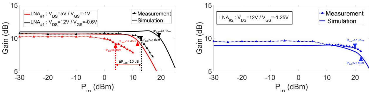
Fig. 5 : Simulated and measured gain vs. RF power at LNAs input for LNA #1 [in its low noise configuration ( V_{DS}=5V / V_{GS}=-1V ), in EM aggression mode ( V_{DS}=12V / V_{GS}=-0.6V )] and for LNA #2 ( V_{DS}=12V / V_{GS}=-1.25V )
