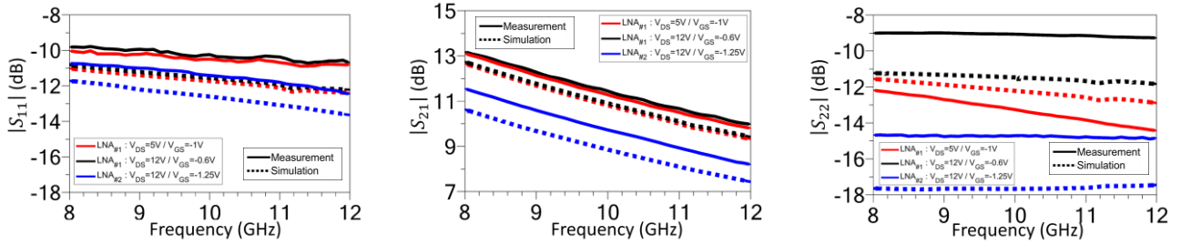
Fig. 4 : Simulated and measured S-parameters of LNA #1 [in its low noise configuration ( V_{DS}=5V / V_{GS}=-1V ), in EM aggression mode ( V_{DS}=12V / V_{GS}=-0.6V )] and of LNA #2 ( V_{DS}=12V / V_{GS}=-1.25V )
