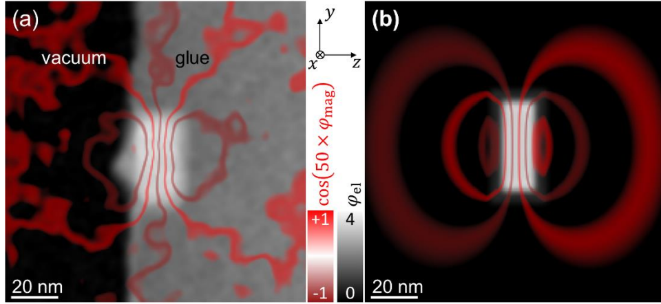
Figure 5. Phase mapping using off-axis EH of the isolated Fe cuboid #5 with a lateral size below 40 nm. (a) Experimental electric phase image (grayscale) superimposed by red isolines of the magnetic phase shift, which correspond to the projected field lines of the magnetic induction. (b) Calculated magnetic phase map from micromagnetic simulation of cuboid #5 displayed in the same way as (a).
