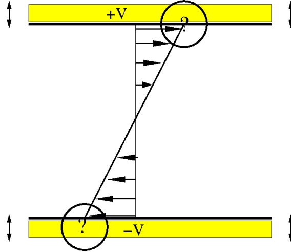
Figure 9. Typical Couette flow.
