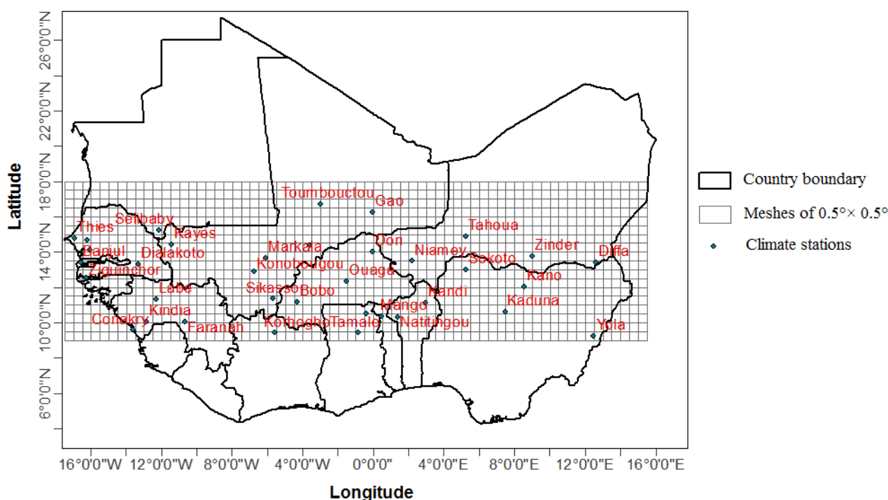
Figure 1. West African Sudano-Sahelian zone and the grids coverage.
