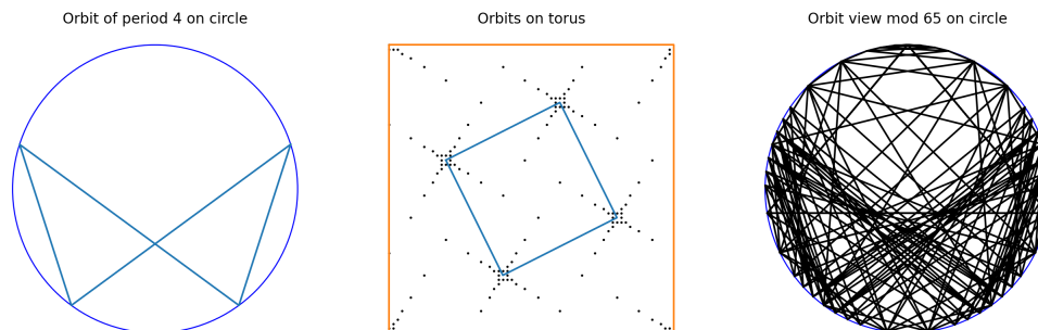
FIGURE 3. In the middle, one sees the orbit of P_N on the torus, for N = 65 = 5F_7 , as well as a square showing the orbit \{(2/5, 1/5), (1/5, 3/5), (3/5, 4/5), (4/5, 2/5)\} . On the left, one sees Launay's representation of this orbit of period 4. And on the right, Launay's representation of the Fibonacci sequence modulo 65.
