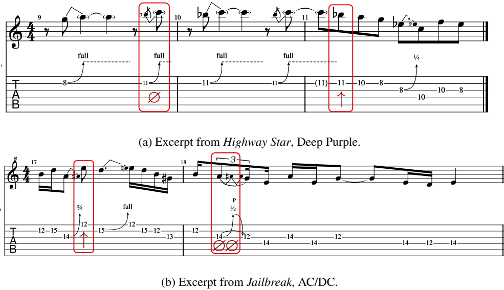
Figure 7: Examples of predictions obtained with our Full Tree model on two different excerpts. Labels shown represent the predicted label for the current note. Only wrong predictions are shown for clarity. All other notes are labeled correctly.
