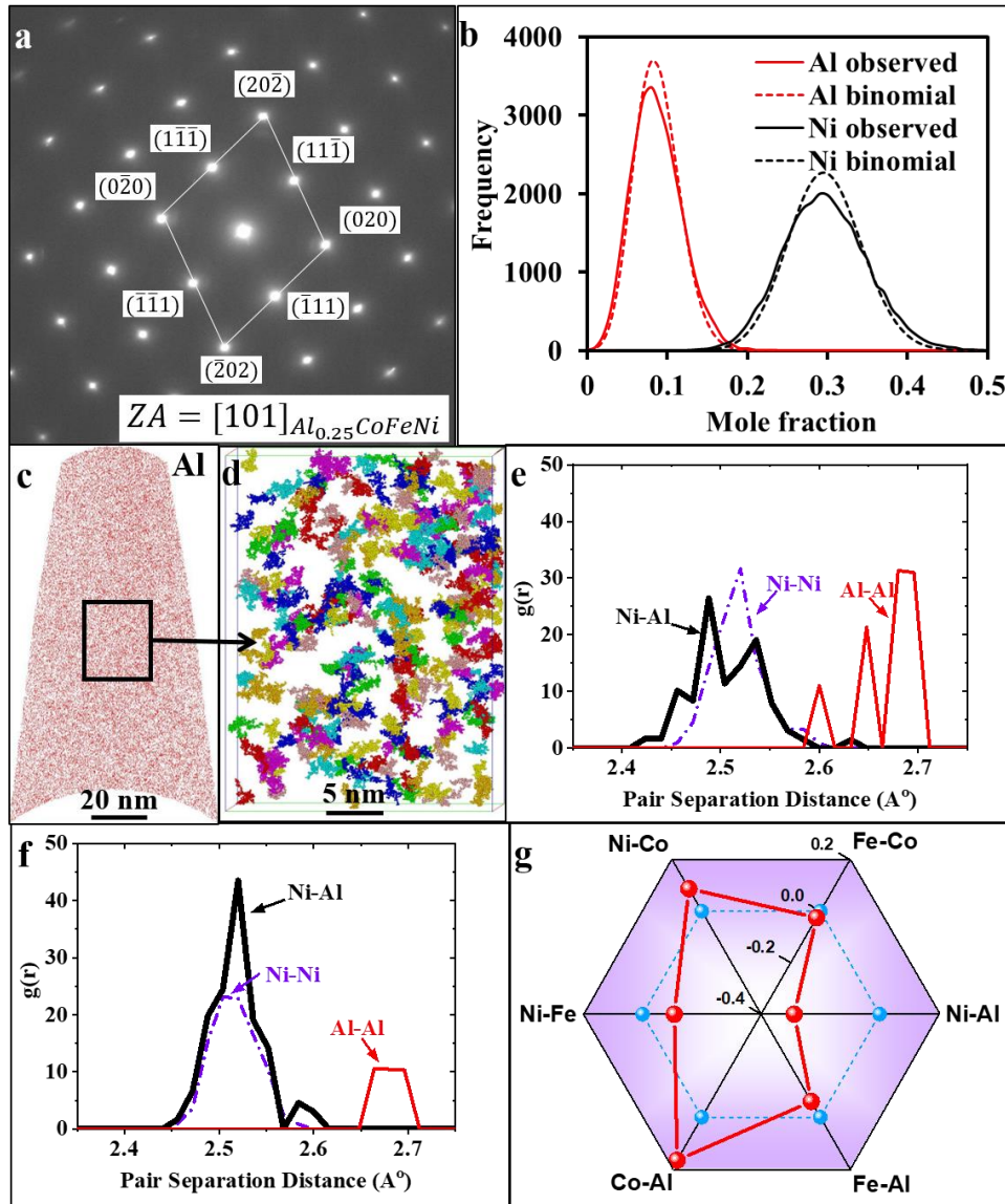
Figure 2: (a-d) Microstructure of \text{Al}_{0.25}\text{CoFeNi} from TEM and APT. (a) SAEDP recorded from [101] FCC zone axis shows only fundamental reflections, indicating the absence of ordering or secondary phases. (b) Frequency distribution of Al and Ni obtained from APT when compared with binomial distributions reveal statistically significant deviations. (c) APT ion map of Al shows uniform distribution. (d) Al-Ni rich clustered-ordering domains are revealed via cluster analysis and are colored differently. (e) Shows pair distribution functions (PDFs) of Ni-Ni, Al-Al, and Ni-Al pairs from 216-atom SQS structure for perfectly random \text{Al}_{0.27}\text{CoFeNi} alloy. (f) Shows PDFs from 216-atom SQS structure for short-range ordered \text{Al}_{0.27}\text{CoFeNi} alloy annealed at 1200^\circ\text{C} . (g) Shows Warren-Cowley SRO parameters ( \alpha_{i-j} ) of various i-j pairs for 1NN shell. The SRO parameters for the perfectly random solid solution and the alloy with SRO at 1200^\circ\text{C} are shown in sky blue and in red, respectively.
