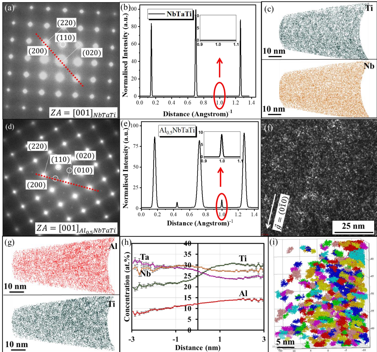
Figure 6: NbTaTi and Al 0.5 NbTaTi microstructural characterization using TEM and APT. (a) SAEDP recorded along [001] BCC zone axis show only fundamental reflections, indicating absence of ordering and/or secondary phases. (b) Intensity profile along the red dotted line in (a) confirms single-phase. (c) Ti and Nb APT ion maps show very early stages of Ti clustering. (d) SAEDP recorded along [001] BCC zone axis showing superlattice reflections, indicating presence
