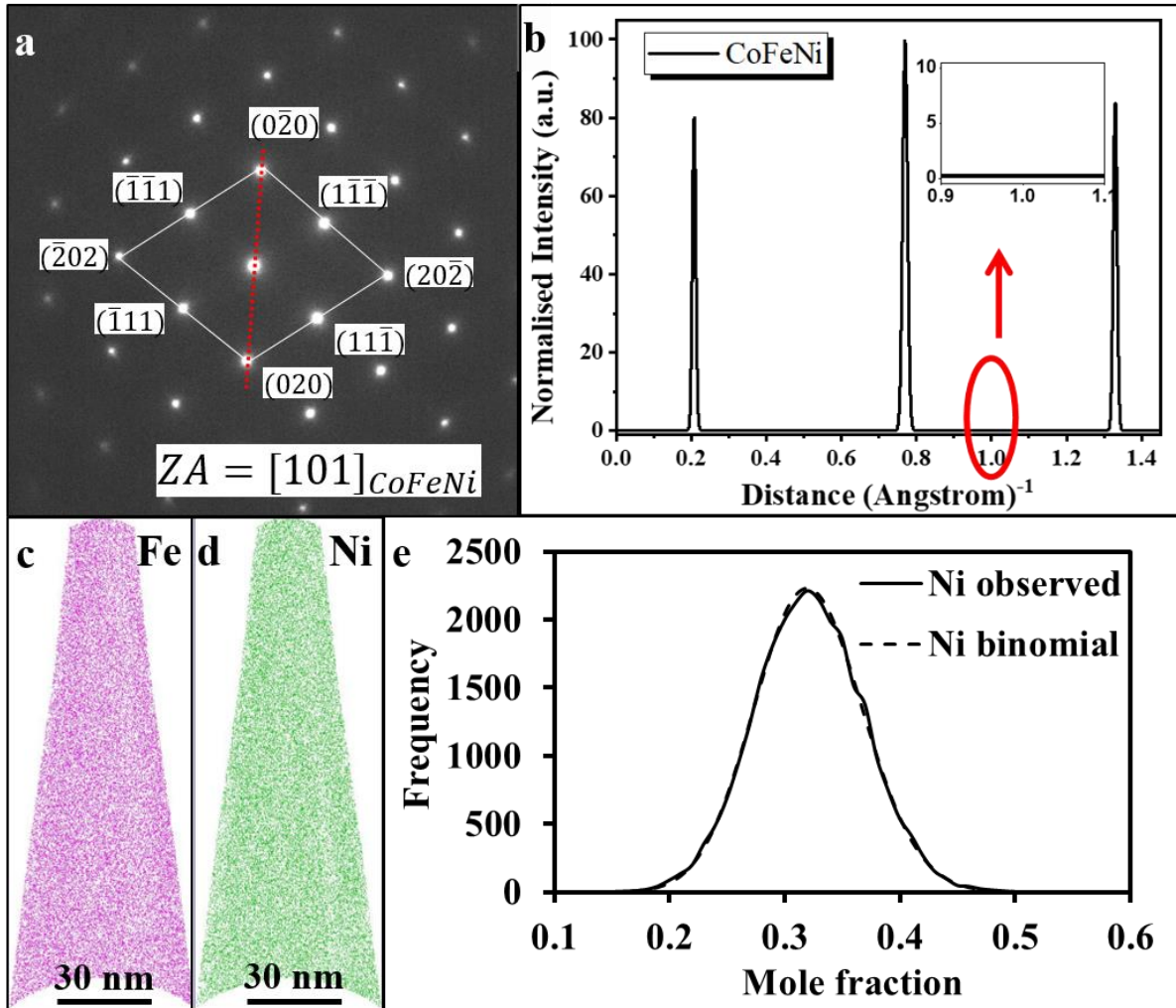
Figure 1: Microstructural characterization of CoFeNi using TEM and APT. (a) SAEDP recorded from [101] FCC zone axis showing only fundamental reflections, indicating absence of ordering or secondary phases. (b) Intensity profile along the red dotted line in (a) confirms single phase microstructure. APT ion maps of (c) Fe and (d) Ni show homogenous distribution. (e) No statistically significant deviation is observed between frequency distribution of Ni obtained from APT and the standard binomial distribution.
