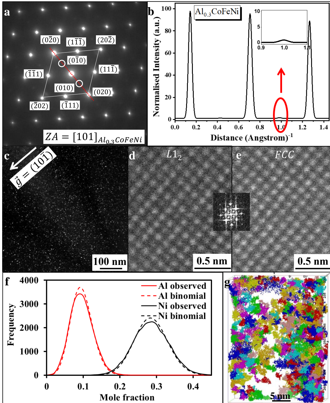
Figure 3: Microstructural characterization of \text{Al}_{0.3}\text{CoFeNi} using TEM and APT. (a) SAEDP recorded from [101] FCC zone axis shows faint superlattice reflections along with fundamental reflections, which indicate ordering. (b) Intensity profile along the red dotted line in (a) confirms ordering. (c) Dark-field TEM micrograph recorded from (10\bar{1}) reflection reveals the ordered domains. HR-STEM micrographs show ordered (d) and disordered (e) structures. Corresponding intensity line profiles along the red dotted lines are shown as bottom insets. (f) Frequency distribution of Al and Ni obtained from APT, compared with the binomial distribution, show significant statistical deviation. (g) Shows Al-Ni rich clusters, obtained from APT.
