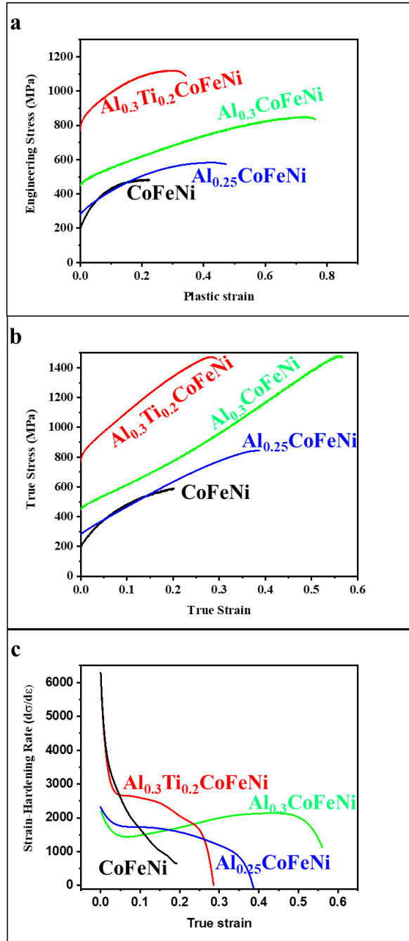
Figure 5: Tensile deformation plots for CoFeNi, Al 0.25 CoFeNi, Al 0.3 CoFeNi, and Al 0.3 Ti 0.2 CoFeNi. (a) Engineering stress-strain curves. (b) True stress-strain curves. (c) Work-hardening rate plots.
