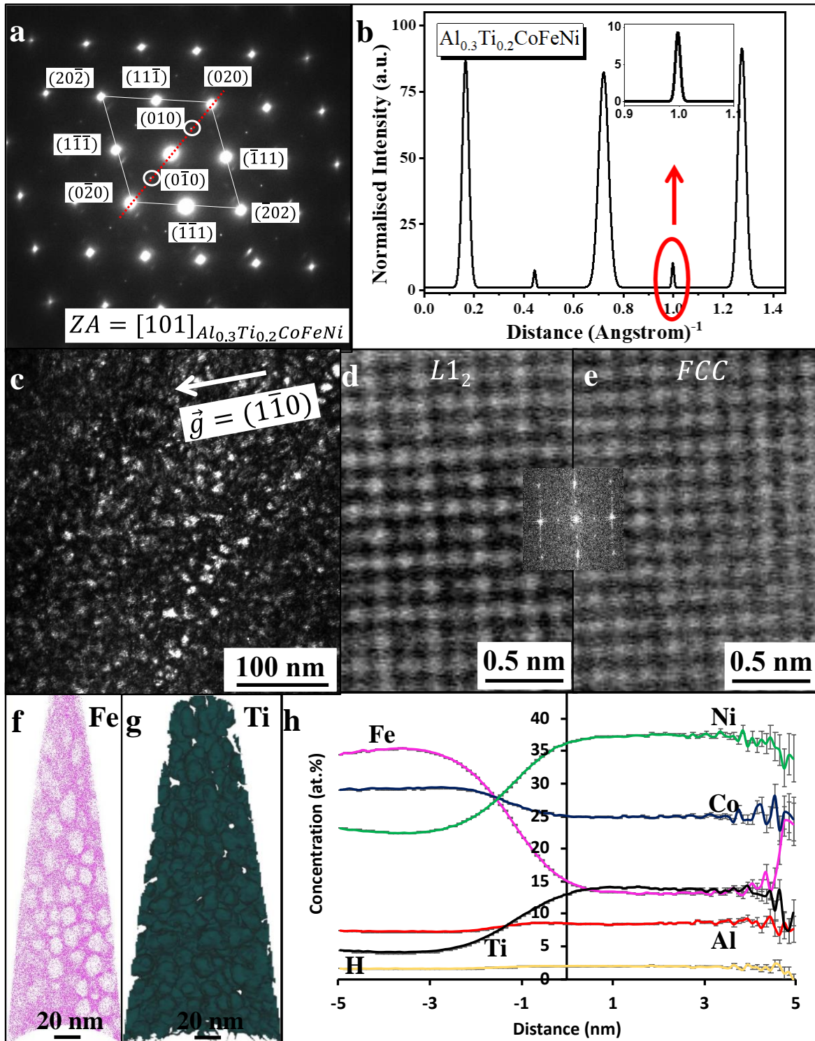
Figure 4: Microstructural characterization of \text{Al}_{0.3}\text{Ti}_{0.2}\text{CoFeNi} using TEM and APT. (a) SAEDP recorded along [101] FCC zone axis shows both sharp superlattice and fundamental reflections, indicating ordering. (b) Intensity profile along the red dotted line shown in (a) confirms ordering. (c) Dark-field TEM micrograph recorded from (1\bar{1}0) reflection reveals ordered domains. HR-STEM micrographs in (d) and (e) show the ordered and disordered structures, respectively. The intensity line profiles along the red dotted lines are shown as bottom insets. (f) and (g) respectively show APT ion map of Fe and Ti. The 11 at.%-iso- concentration surface shows Ti rich LRO domains. (h) Proximity histogram show the elemental partitioning between FCC matrix and LRO domains. Error bars colored gray.
