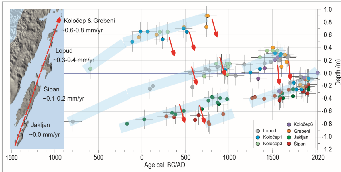
Fig. 10 Relative sea-level changes at the Elafiti islands (Lopud, Koločep, Grebeni – Faivre et al., 2021a,b; and Jakljan and Šipan – this study) based on the geochronology of algal rims. Error bars correspond to two standard deviations ( 2\sigma ). Blue band represents segmented linear trendlines. Red arrows mark periods of abrupt RSL fall i.e., possible seismic events. Left: dashed red arrow point to active coastal sectors in the past 1.6 ka with increasing uplift rates. Zero relates to the time of sampling at a particular location between 2016-2020.
