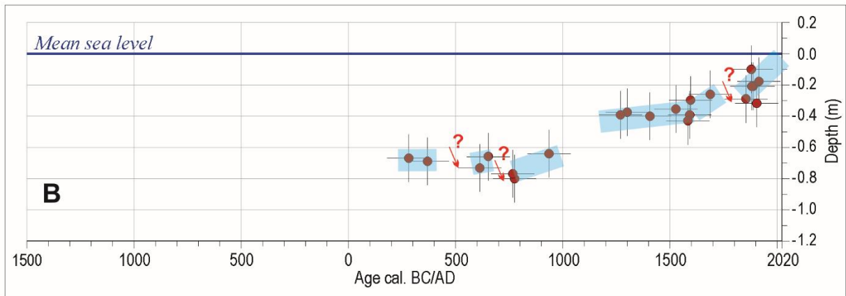
Fig. 4 Relative sea-level changes at Šipan island; A) algal rim; B) 1.8 ka RSL curve derived from the algal rims - red circles. Error bars correspond to two standard deviations (2s). Blue band represents segmented linear trendlines. Red arrows mark periods of abrupt RSL change i.e. potential coseismic events.
