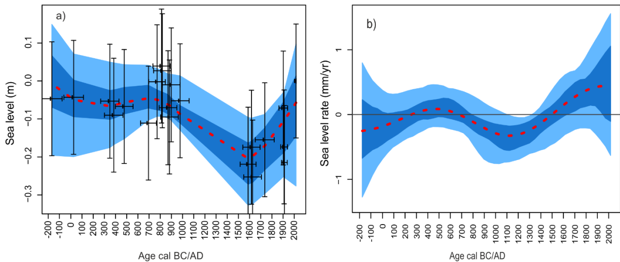
Fig. 5 A) GIA adjusted sea-level change for Jakljan Island, EIV-IGP model predictions (mean (dashed red lines) with 68% (dark blue) and 95% (light blue) confidence intervals); B) Estimated rates of sea-level change after GIA correction.
