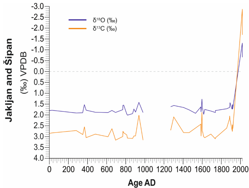
Fig. 6 Stable isotopes records from the Šipanj and Jakljan algal rims.
