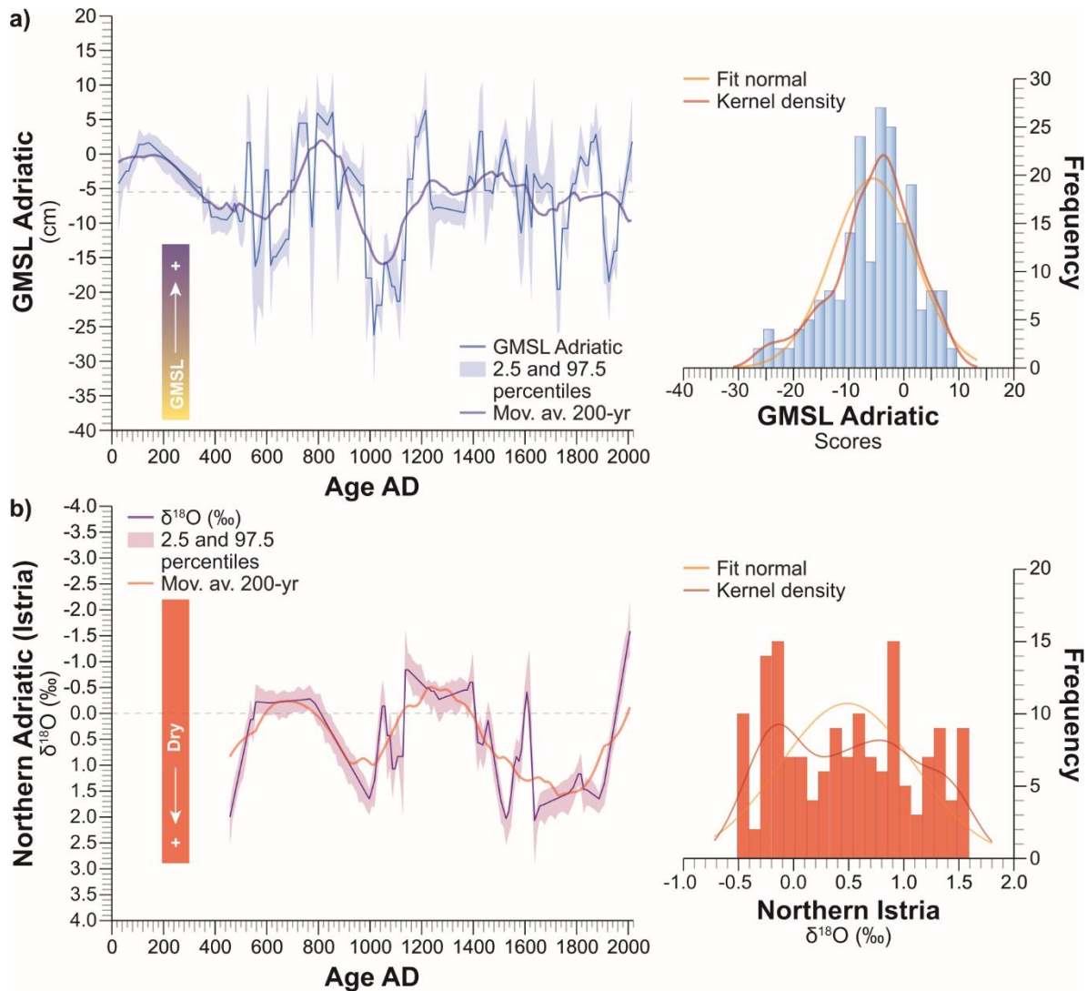
Fig. 7 a) Variation of global mean sea-level contribution (GMSL) from the Adriatic during the last two millennia. b) Northern Adriatic \delta^{18}\text{O} ‰ VPDB records from algal rim structures (Faivre et al., 2019a). The two curves are shown with a 95% confidence band (2.5 and 97.5 percentiles). The long-term trends are depicted as a 200-yr moving average. The frequency distributions are portrayed with a normal Fit and Kernel density estimations.
