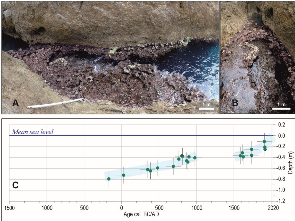
Fig. 3 Relative sea-level change at Jakljan island; A) and B) algal rim, C) 2.2 ka Relative sea-level curve derived from the algal rims - green circles. Error bars correspond to two standard deviations (2s). Blue band represents segmented linear trendlines.
