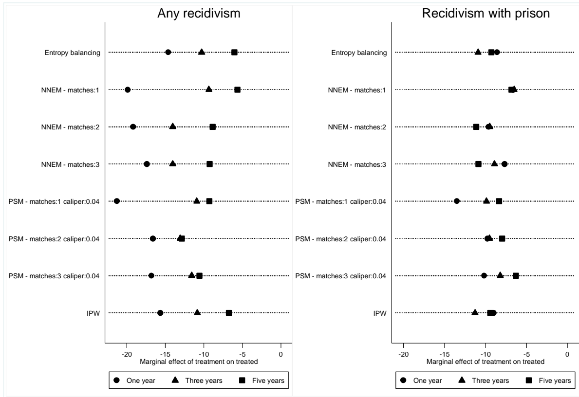
Figure 5. Marginal effect of SL on recidivism using different matching methods
