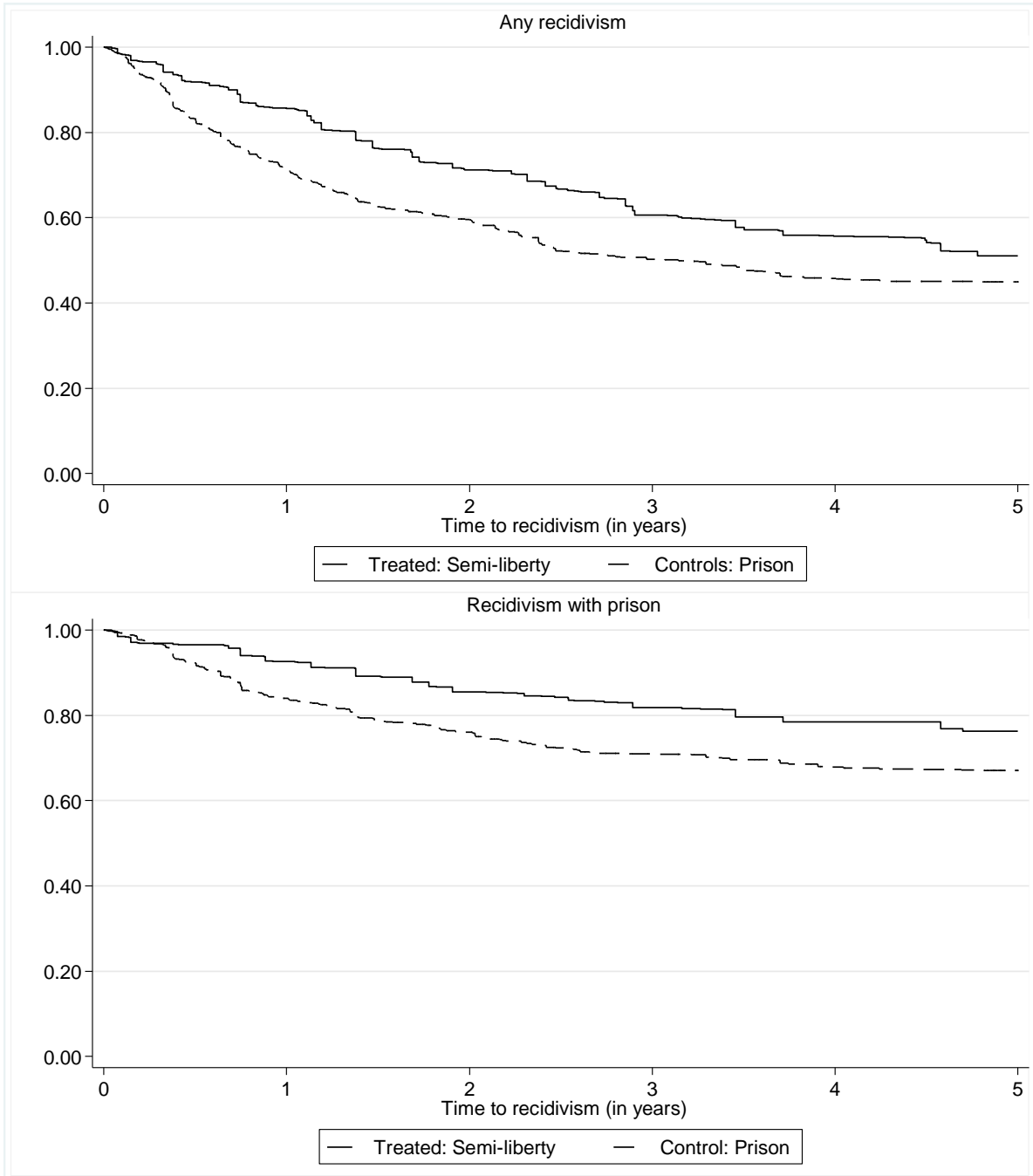
Figure 4. Marginal effect of SL on hazard rate of recidivism after entropy balancing
