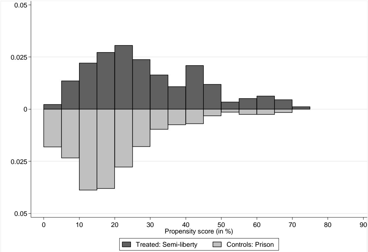
Figure 3. Distribution of estimated propensity scores for SL and non-SL offenders
