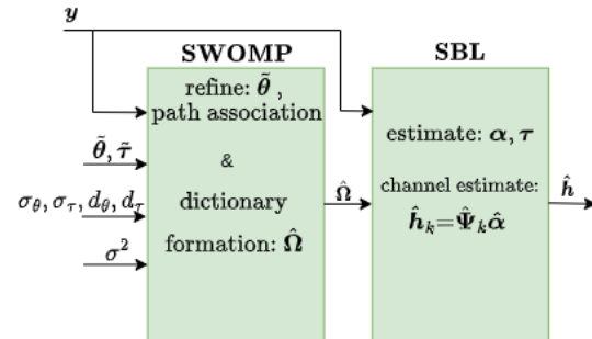
Fig. 4. SWOMP-SBL algorithm.
