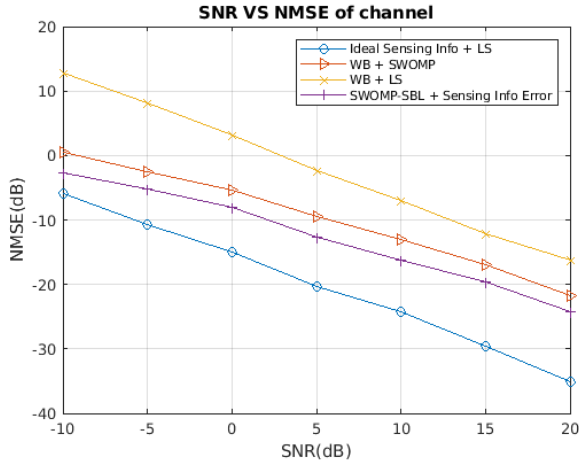
Fig. 6. SNR vs NMSE of the channel estimates.
