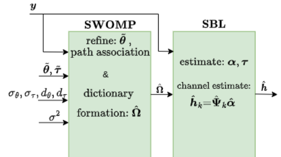
Fig. 4. SWOMP-SBL algorithm.
