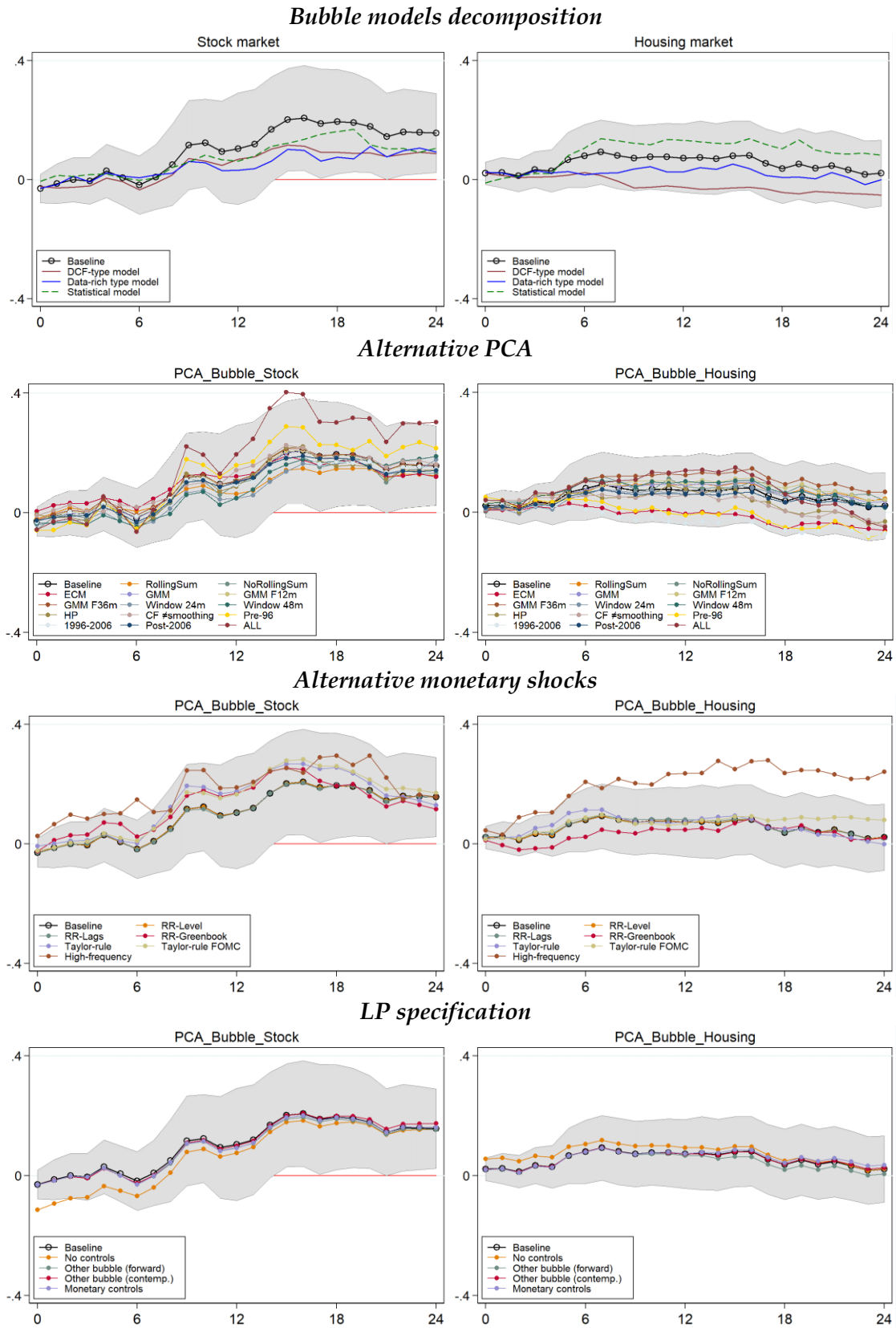
Figure A. Robustness tests for the linear specification
