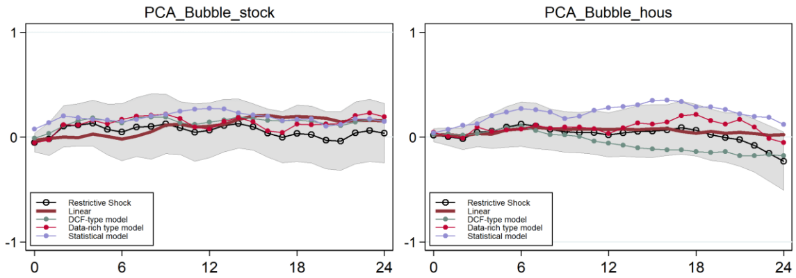
Figure B. Robustness tests to the non-linear specification
