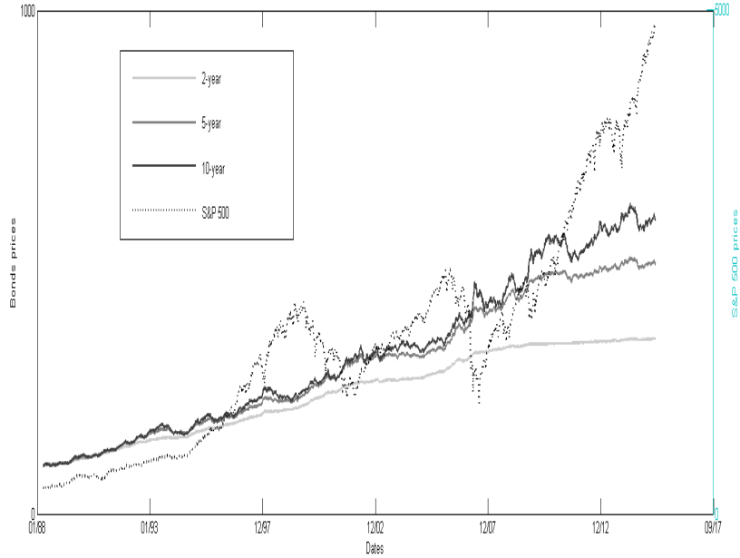
Figure A.1: Dynamics of asset prices
