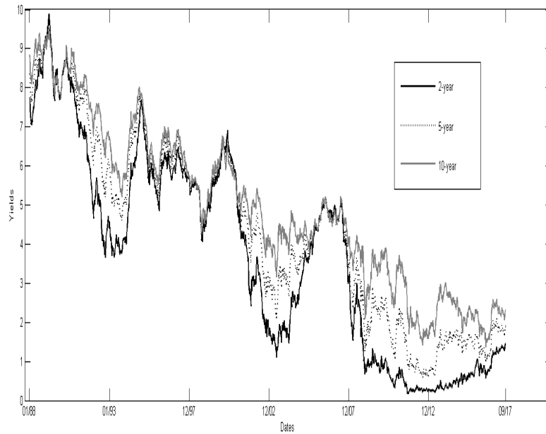
Figure A.2: Dynamics of US government bond yields
