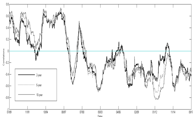
Figure 1: Rolling-window estimates of US stock-bond correlation
