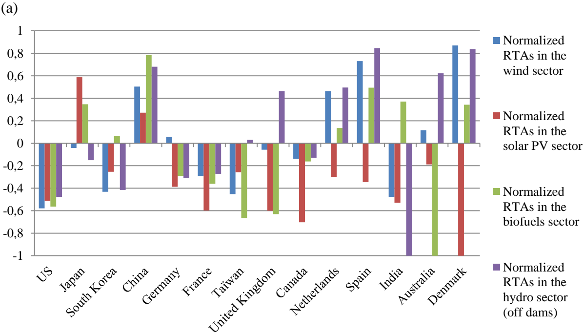
Figure 3 : Evolution of the normalized RTA indices (a) 1992-2003 period (b) 2004-2014 period
