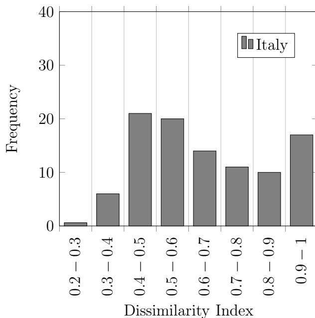
Figure 2: Dissimilarity Indices
