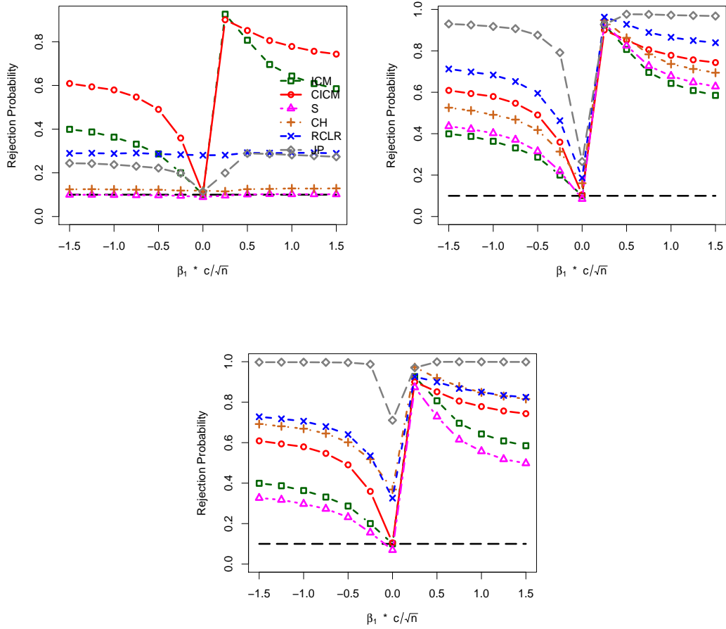
Figure 3: Power curves for Group Heterogeneity Model (iii): benchmark 1 IV (top left), 7 IV (top right), and 15 IV (bottom).
