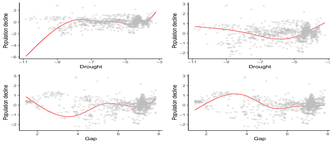
Figure 4: Generalized additive model explaining population collapse by a univariate function of the two reliable climate instruments, drought (top panel) and gap (bottom panel) by region for the 2 largest regions, NE (left panel) and NG (right panel).
