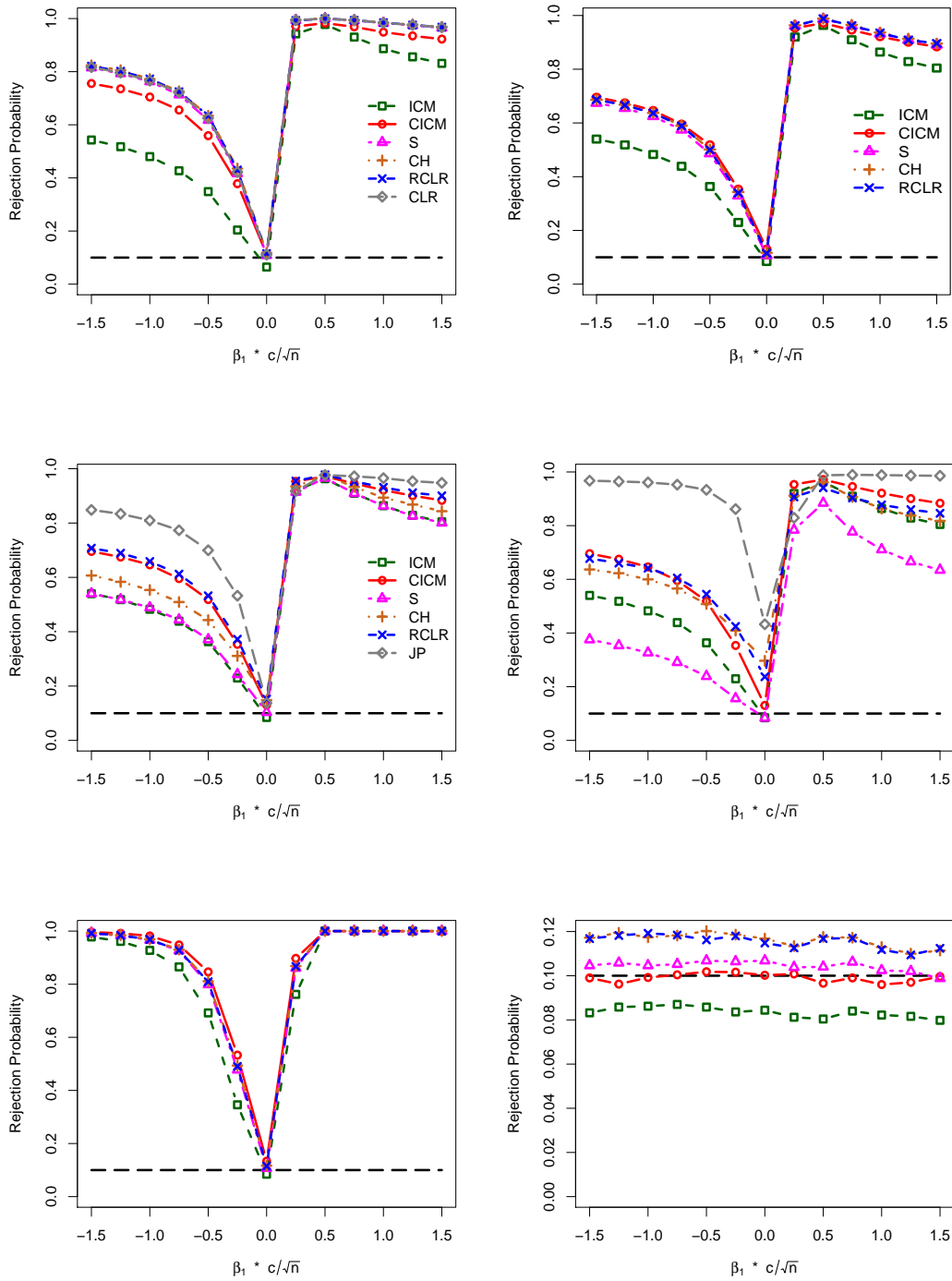
Figure 2: Power curves for Linear Model (ii): homoskedastic case (top left), benchmark heter. 1 IV (top right), heter. 3 IV (middle left), heter. 7 IV (middle right), stronger identification (bottom left) and no identification (bottom right).
