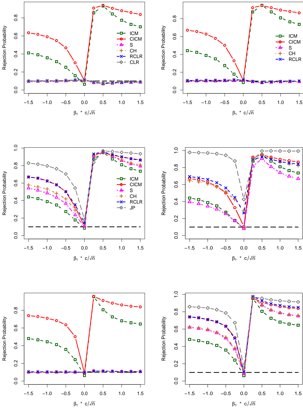
Figure 1: Power curves for Polynomial Model (i): homoskedastic case (top left), benchmark heter. 1 IV (top right), heter. 3 IV (middle left), heter. 7 IV (middle right), heter. 1 IV with sample size 401 (bottom left), and heter. 3 IV with sample size 401 (bottom right).
