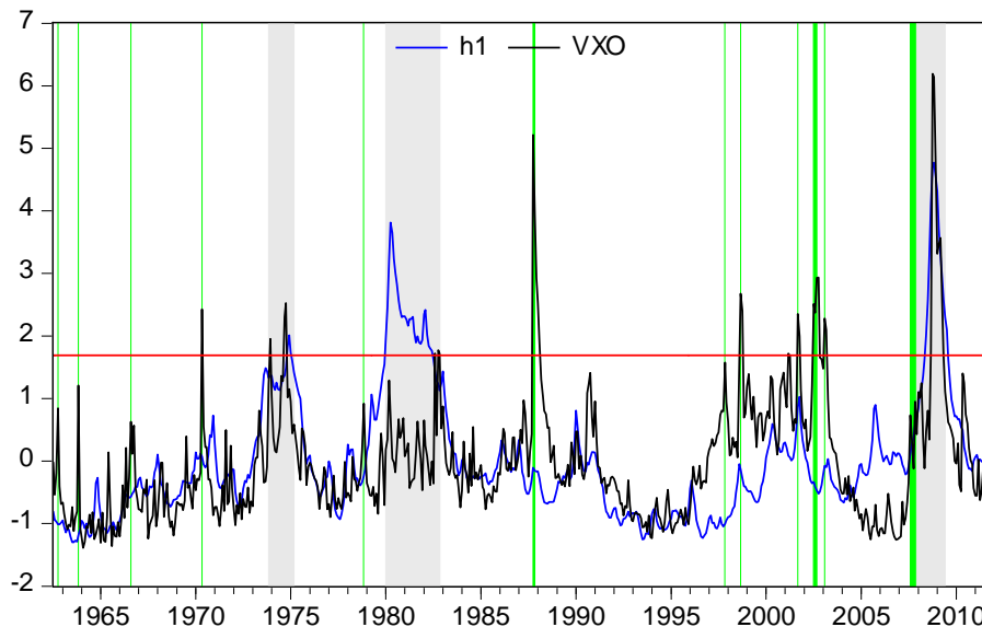
Figure 2: Bloom (2009)'s index vs. Jurado et al. (2014)'s measure for uncertainty
