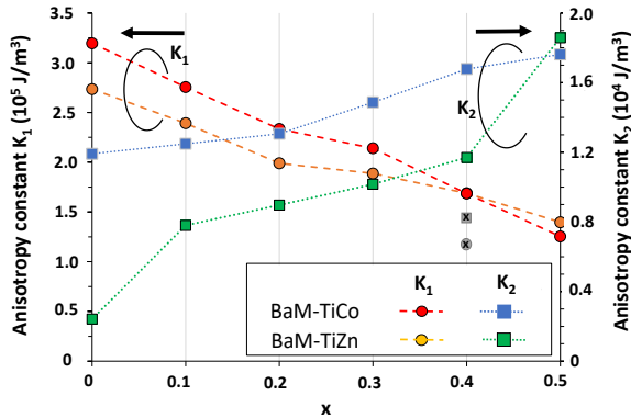
Fig. 7. First and second order anisotropy constants plotted against the doping level x. Symbols in grey are data extracted from [13].
