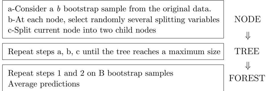
Figure 1: RF Algorithm
