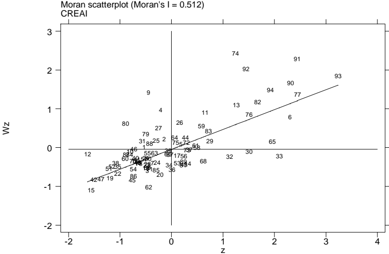
Graph 3 – Moran’s diagram for the normalized value of entry rate ( CREAI )
