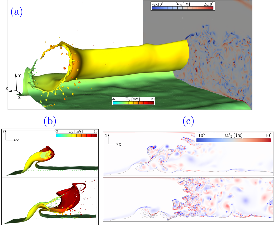
FIG. 3. (a) An isometric view of that bag morphology resulting from the shearing of a thin film of thickness \mathcal{H}_f = 1\text{mm} within the cough machine. Side-walls of the rectangular channel ( cough-machine ) are not shown for the ease of visualization. The shearing velocity used in the 3D computations is 15 m/s. A vorticity map shown on the vertical cross-section (grey panel) highlights the flow structure around the inflated liquid bag. (b) Snapshots illustrating the inflation and atomization of a liquid bag observed in 3D simulations. (c) Side-view of bag-breakup mode observed in 2D simulations. All computations are performed using Basilisk .
