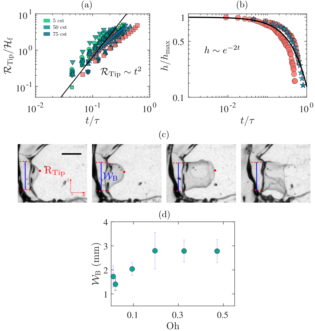
FIG. 4. (a) Kinematics of bag expansion measured for different film viscosities \nu = 5 cst, 50 cst and 75 cst. Symbols are color coded according to the film viscosity. Data from 3D simulations ( \star = 15 m/s) and 2D numerical simulations ( \bullet = 30 m/s and \blacksquare = 15 m/s) are performed for film viscosity \nu = 5 cst. Solid black line is theoretical prediction for bag-inflation kinematics, \mathcal{R}_{\text{Tip}} \sim t^2 . (b) Theoretical exponential decay in bag thickness, h \sim e^{-2t} (solid black line), measured in numerical computations. Here, the bag-thickness is non-dimensionalised by its maximum value. (c) Sequence of experimental snapshots illustrating the fact that the width of the bag \mathcal{W}_B at the location of the attachment with the crest of the interfacial wave remains nearly constant while it inflates. The vertical lines on each snapshot corresponds to the instantaneous width of the bag. The horizontal scale-bar shown on the first snapshot corresponds to 1 mm. (d) Experimentally measured variation in bag width with film viscosity. The data corresponds to experiments performed with film thickness \mathcal{H}_f = 1 mm and U = 30 m/s.
