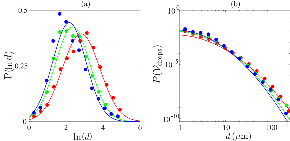
FIG. 7. Droplet size distribution measured at 10 cm away from the the exit of the channel. (a) Size statistics measured for different film viscosity \bullet = 5 cst, \bullet = 25 cst and \bullet = 105 cst. For these measurements the flow velocity and film thickness was fixed at U = 30 m/s and \mathcal{H}_f = 1 mm. Solid lines are a log-normal fit to the data. (b) Volume based size statistics measured for different film viscosities. Solid lines are corresponding log-normal fits to the data.
