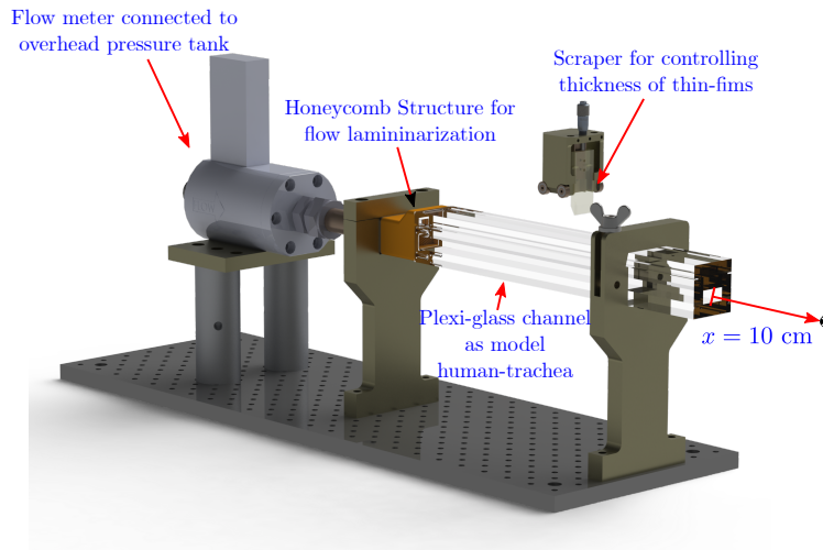
FIG. 1. Schematic diagram of the experimental setup. A transparent plexi-glass channel with rectangular cross-section (model-trachea) is connected with a pressurized tank via a valve. A thin layer of aqueous glycerol solutions covers the bottom of the channel. Upon actuation of the valve, the events leading to the fragmentation of thin-film are recorded by a high-speed camera in top view. Droplet statistics are measured at a distance of 10 cm away, along the center-line, from the exit of the channel.
