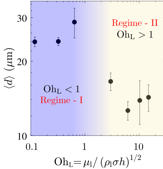
FIG. 9. Experimentally measured variation in the mean droplet size \langle d \rangle with local Ohnesorge number Oh_1 = \mu/(\rho \sigma h)^{1/2} . The length scale in Oh_1 is the typical bag-thickness h \sim 1 \mu\text{m} . In Regime-I, Oh_1 < 1 a balance between inertia and capillary forces decides the eventual fate of a bag, causing it rupture early, whereas in Regime-II, Oh_1 > 1 viscous effects enhance the stability of the thin sheets, causing it to burst at later times, thus producing smaller droplets.
