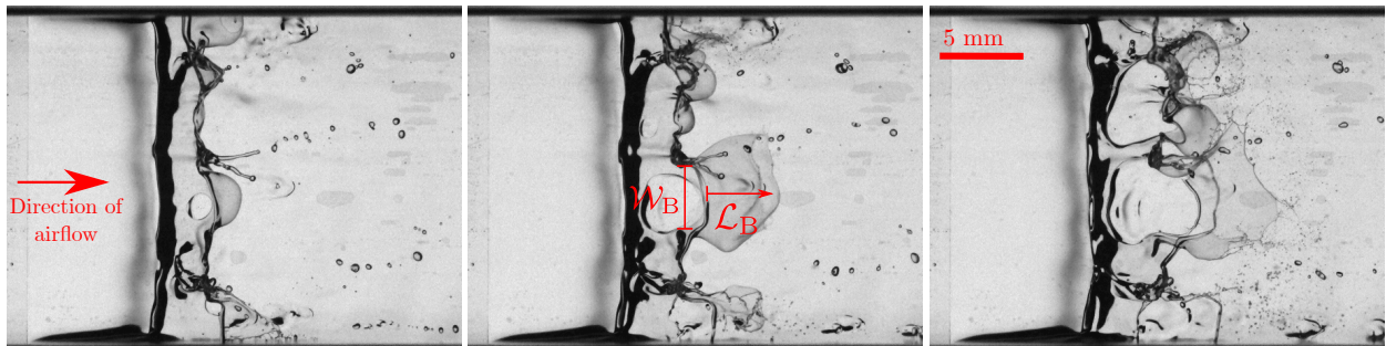
FIG. 2. Sequence of experimental snapshots, at 0.25 ms intervals, highlight the key processes during the fragmentation of a thin-film of water-glycerol solution (film thickness \mathcal{H}_f = 1 \text{ mm} and kinematic viscosity \nu_1 = 5 \text{ cst} ) when sheared by an impulsively started airflow in a cough-machine. The mean velocity of the airflow is 15 m/s. The sequence shows the topological changes experienced by the film as multiple bags form along its width. The disintegration of these inflated structures generates droplets with broad size statistics. The first snapshot is captured 40 ms after the initiation of airflow in the channel.
