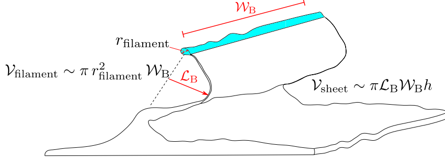
FIG. 6. A schematic comparing the volume accompanying the inflated liquid sheet and the filament bordering the inflated morphology.
