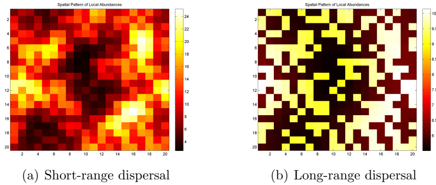
Figure 8: Effect of dispersion parameters on spatial abundance pattern
