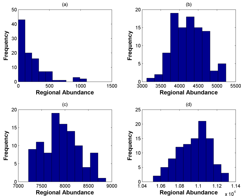
Figure 5: Frequency distribution of regional abundance for economic contexts: (a) \mathcal{E} = 4.57 , (b) \mathcal{E} = 6.40 , (c) \mathcal{E} = 8.23 , (d) \mathcal{E} = 10.07 .
