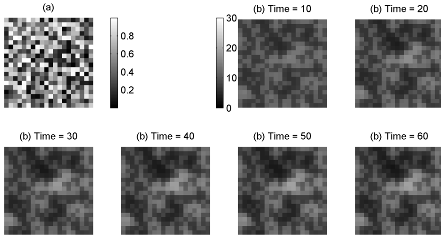
Figure 3: (a) Soil Quality Map (b) Population dynamics snapshots for various times and a landscape half-made of grassland. Parameters : r_C = -0.1, r_G = +0.1, \beta = 0.25, \sigma = 1, K = 30, N_{thresh} = 2
