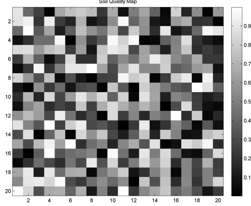
Figure 1: An example of soil quality map - The soil quality of each field i , Q_i is drawn with uniform probability distribution in [0, 1] .
