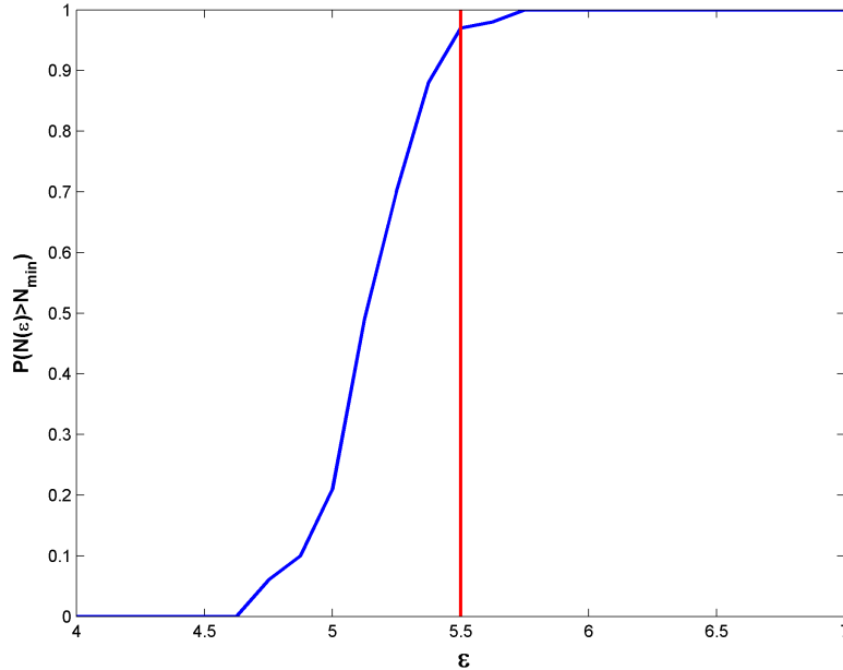
Figure 7: Probability to achieve the conservation objective with respect to the economic context: \mathbb{P}(\lim_{t \rightarrow \infty} N_t(\mathcal{E}) \geq N_{min})
