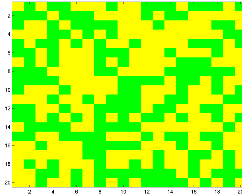
Figure 2: Landscape resulting from agricultural land use. Fields G are green (/dark) and C are yellow (/clear). That landscape has been obtained by comparing the soil quality, Q_i , to 0.5
