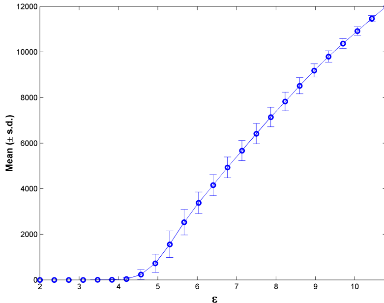
Figure 6: Expected ( \pm standard deviation) regional abundance N w.r.t. the economic proxy \mathcal{E}
