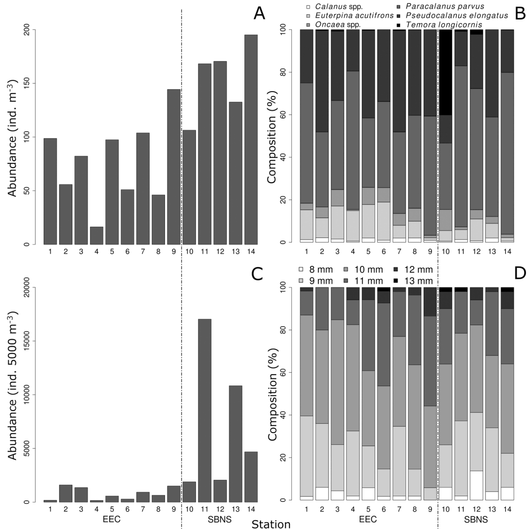
Fig. 2. Abundance distribution of (A,B) 6 dominant copepod species (ind. m^{-3} ) and (C,D) Downs herring larvae (ind. 5000 m^{-3} ) by size (mm) during winter 2014 (January–February) in the Eastern English Channel (EEC) and the Southern Bight of the North Sea (SBNS). Only stations where larvae were collected for gut analyses are shown
