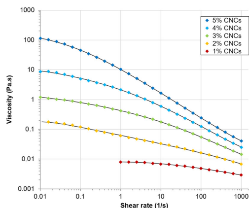
Figure 7. Steady-state viscosity (Pa·s) of CNCs suspensions with concentration ranging from 1 to 5% ( w/w ) as a function of shear rate (1/s). Black lines represent data fitted with the Carreau–Yasuda model.
