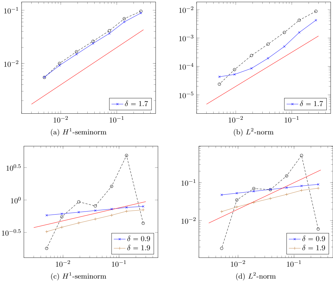
Figure 5: Test-case 2. Relative errors vs. h for \nu = -10.57 (top) and \nu = -2.1 (bottom). Dotted black: cFE, Solid blue/brown: optimization-based, Solid red: h^\kappa for H^1 , h^{\kappa+\frac{1}{2}} for L^2 .
