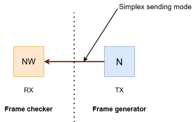
Figure 5. A simplex mode implemented on GTX transceivers as first-stage protocol to communicate between two adjacent Wizard tiles.
