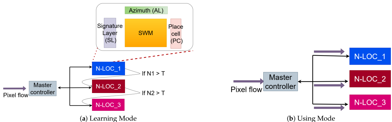
Figure 7. Expanding bio-inspired neural network architecture N-LOC over Wizardre multi-tiles. In the learning phase, the data-copy of each current landmark will be held on one bloc IP. If the number of learned neurons in N-LOC1 is overloaded (superior to a fixed threshold T ), we will switch into next available bloc IP which is the second one. Then, it will be the same rule for all different bloc IPs. In process phase, all bloc IPs works simultaneously, the best score among the three represents the accurate and appropriate localisation of a given image.
