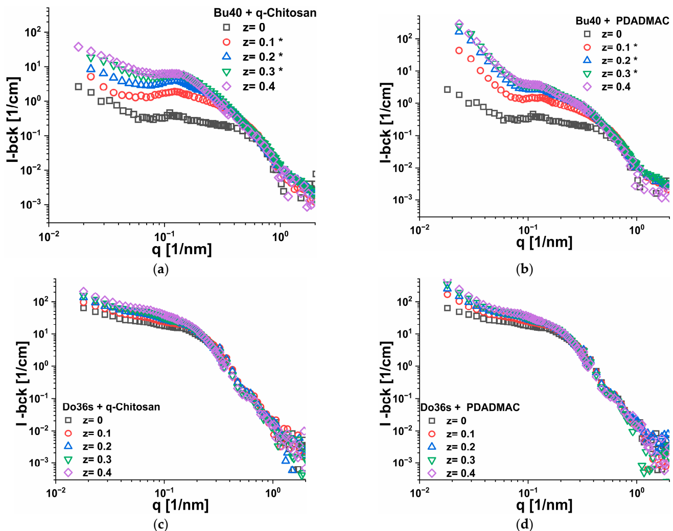
Figure 6. SANS intensity as a function of q for all z ratios from 0 to 0.4 for samples of 5\text{ g/L} (a,b) \text{nBu}_{40}\text{-b-AA}_{167} (Bu40) or (c,d) \text{nDo}_{36}\text{-b-AA}_{71} (Do36s) complexed with different amounts of either q-chitosan or PDADMAC (data from LLB which were corrected with respect to HZB data and ones from HZB which are marked as *. see Supplementary Materials Section S6.2).
