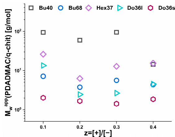
Figure 5. The ratio of apparent molecular weight ( M_w^{app} ) of the IPECs obtained by complexing solutions of 5 g/L AlkA-b-NaPa with different amounts of polycation from SLS experime.
