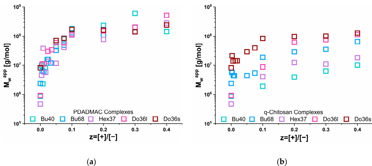
Figure 4. The apparent molecular weight ( M_w^{app} ) of the IPECs obtained by complexing solutions of 5 g/L AlkA-b-NaPa with different amounts of polycation (a) PDADMAC or (b) q-Chitosan via SLS.
