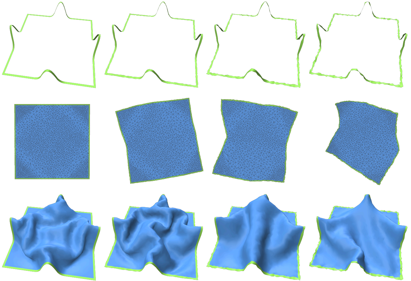
Fig. 10. Influence of noise in the flattening of the hole boundary (second row) and the resulting hole filling (third row). Each vertex of the input mesh has been randomly shifted by a 3D vector uniformly sampled in the unit square times \sigma (first row). The first column is free of noise, the second represents the result for \sigma , the third for 2\sigma and the last for 3\sigma .
