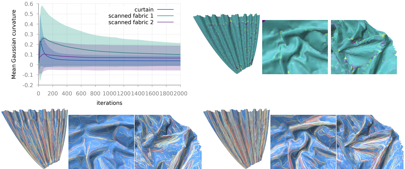
Fig. 8. Graph showing the evolution of the average Gaussian curvature and its variance on Curtain , Scanned Fabric 1 and Scanned Fabric 2 as a function of the number of iterations in the minimization process of the developability energy. The initial values are computed after applying ARAP. The top right figures show the distribution of the Gaussian curvature on the meshes. The bottom figures show the directions of minimum curvature (ruling directions) for respectively the initialization after ARAP and the minimization of our energy.
