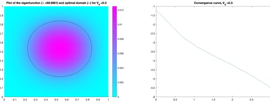
Figure 2: V_0 = 0.3 . Left: representation of the optimal domain (black contour) and the eigenfunction (warmer colors indicate where the function takes its maximum values). Right: evolution of the quantity \|f_{k+1} - f_k\|_{L^1(\Omega)} as a function of iterations, on a logarithmic scale.
