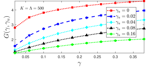
Fig. 2: Multiplicative gap G(\gamma, \gamma_u) between \bar{T}(\gamma, \gamma_u) from (16) and T_{\min}(\gamma, \gamma_u) from (17).
