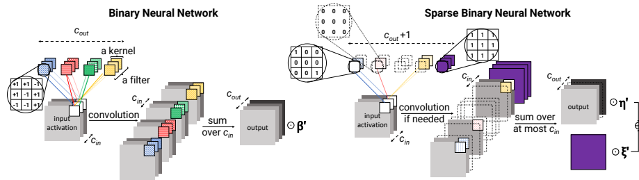
Fig. 1: BNNs vs. SBNNs operations in a convolutional layer using c_{out} filters and input of c_{in} dimensions. BNNs’ (c_{out} \cdot c_{in}) convolutional kernels are dense and require all computations. SBNNs’ kernels are sparse, allowing to skip certain convolutions and sum operations. The removed filters are indicated by a dashed contour and no fill. Both BNNs and SBNNs perform convolutions using XNOR and popcount operations, while the sum is replaced by popcount operations.
