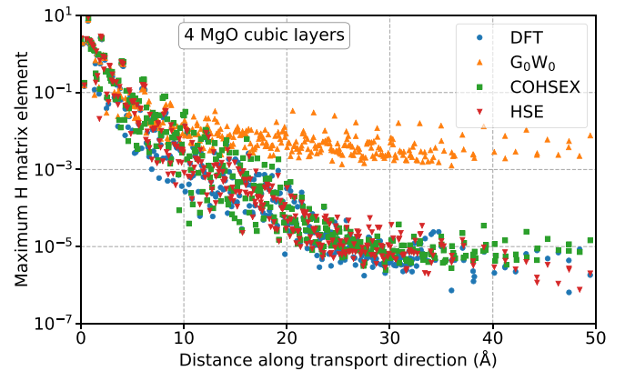
FIG. 2. Maximum modulus of the Wannier Hamiltonian matrix elements (7) as a function of the distance between Wannier centers along the transport direction, as calculated by various approximations, here shown for the longest system (4 Ag/4 MgO/4 Ag). The difference between DFT and G_0W_0 is only due to the change of eigenvalues in Eq. (4). On the contrary, for HSE and COHSEX, the matrix U_{mn}^{(k)} also changes.
