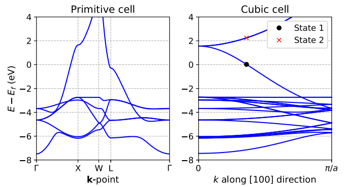
FIG. 13. DFT-PBE band structure of bulk Ag, either computed in the primitive cell, or in the cubic cell along the [100] direction ( \mathbf{k}^{\parallel} = 0 ). a is the lattice parameter.
