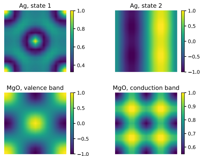
FIG. 14. Color maps of some Bloch wave functions at \mathbf{k}^{\parallel} = 0 in a (xy) slice of the cubic cell. State labeled 1 on the band structure plot (Fig. 13) has symmetry \Delta_1 while state labeled 2 has symmetry \Delta_2 (it is doubly degenerate, the other one having mirror symmetry along the horizontal axis). The highest valence states and lowest conduction states of MgO both have \Delta_1 symmetry.
