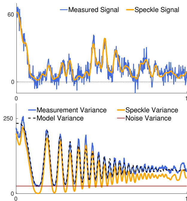
Fig. 10. Illustration of the simulation environment. The top image represents a speckled measurement before and after the addition of the noise. The bottom image represents both the empirical and model variances used within RIM-VAR, in the case where 500 speckles have been generated. It is noticeable that the empirical variance is roughly the speckled variance shifted by a fixed amount (here, roughly 25), corresponding precisely to the variance of the additive noise plaguing the data. With 500 speckles, there remains significant differences between the empirical variance and the model variance.
