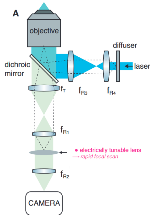
Fig. 9. Remote focusing setup used for the acquisition of the data presented in Fig. 4
