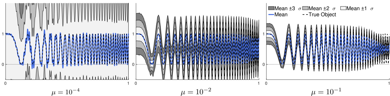
Fig. 12. Statistical result of Monte-Carlo reconstruction with RIM-STD
