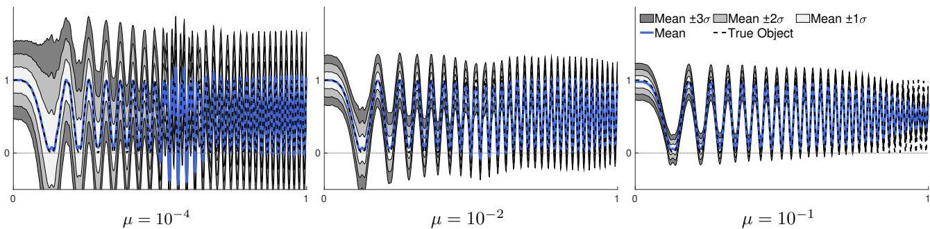
Fig. 13. Statistical result of Monte-Carlo reconstruction with RIM-CF, after data pre-filtering
