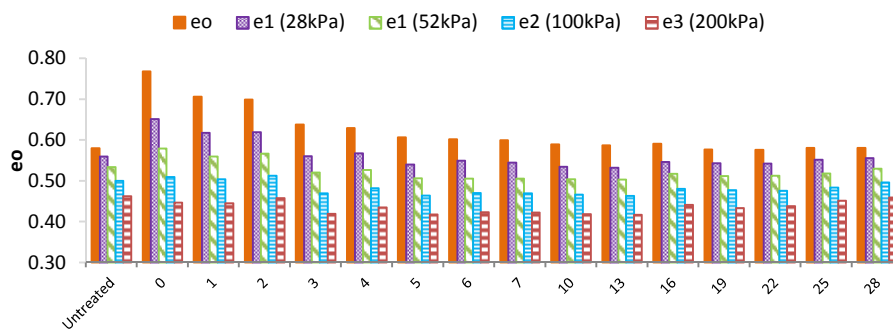
Figure 5. Evolution of the void ratio overtime
