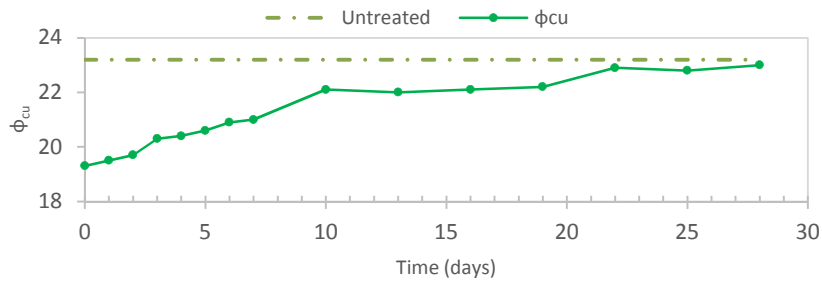
Figure 9. Evolution of the internal friction angle over the time
