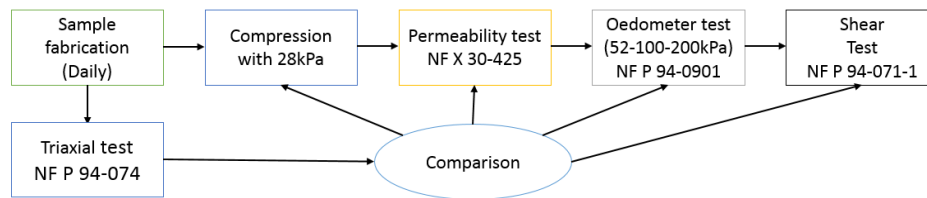
Figure 1. Methodology for the experimental campaign
