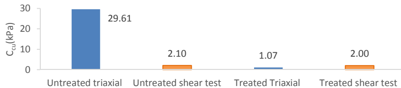
Figure 11. Change of cohesion (28 days, Triaxial and shear tests)
