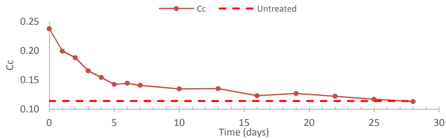
Figure 8. Evolution of the compressibility coefficient over time
