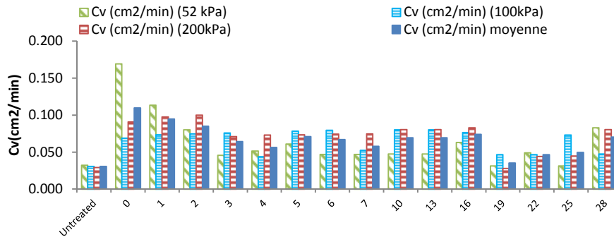
Figure 7. Evolution of the consolidation coefficient over the time
