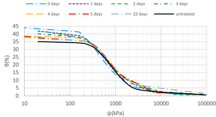
Figure 4. Evolution of the untreated soil water retention curve
