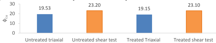
Figure 10. Change of the internal friction angle (28 days, Triaxial and shear tests)
