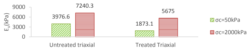
Figure 12. Change of the undrained modulus (28 days, Triaxial and shear tests)
