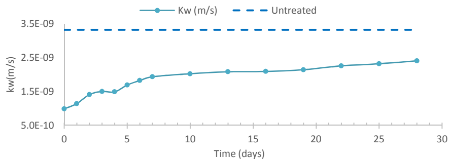
Figure 3. Evolution of the permeability over time
