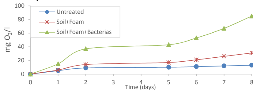
Figure 2. Degradation test results with spirometer (T.Vogel)
