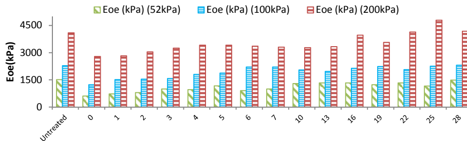
Figure 6. Evolution of the oedometer modulus
