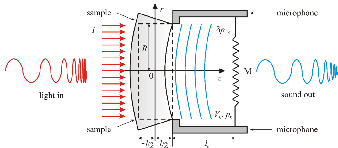
Figure 3. Scheme of a LTI for the photoacoustics thermoelastic frequency response. The red and blue lines represent the sinusoidal input (modulated light) and output (sound) signals oscillating at the same frequencies, as processed by an open photoacoustic cell.
