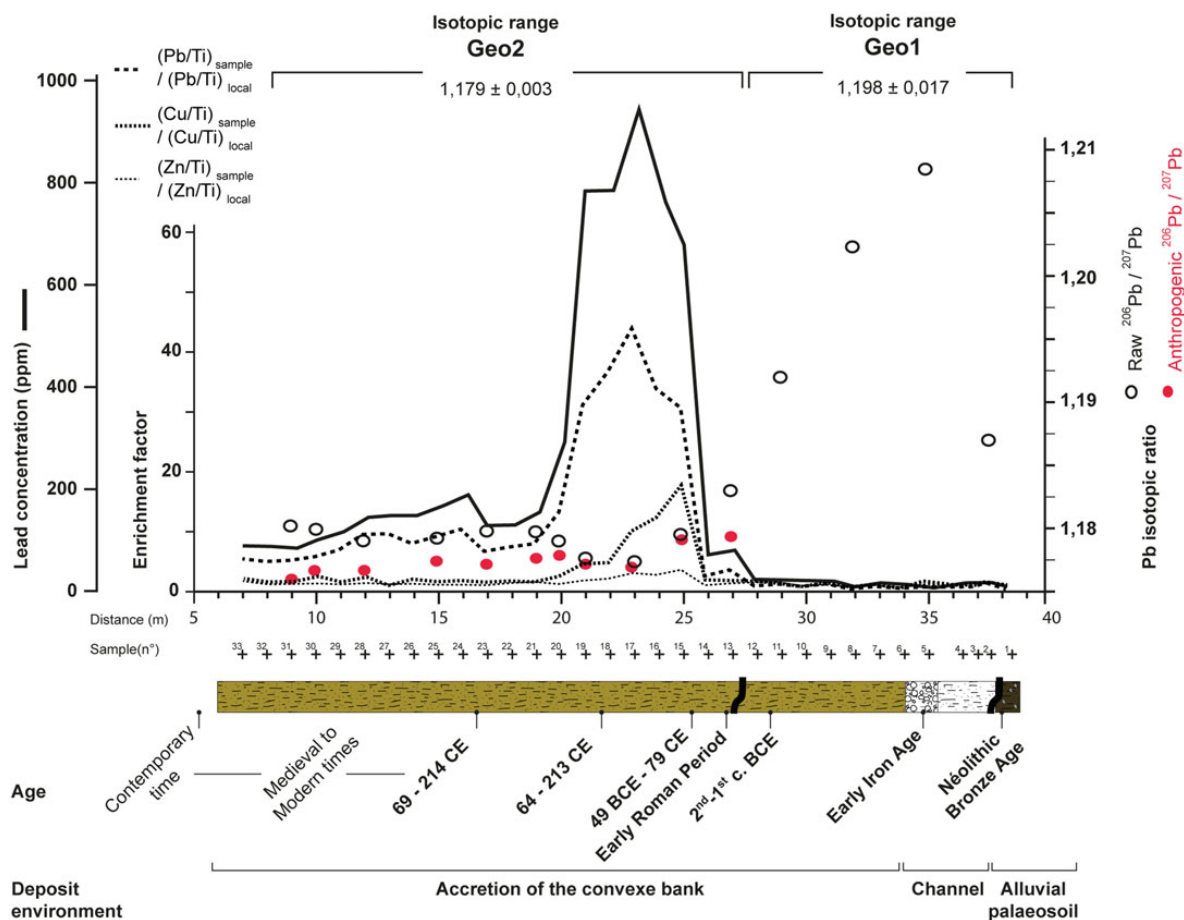
Fig. 4. Synthetic stratigraphic log of the site showing chronology, Pb concentration (ppm), Pb, Cu, and Zn enrichment factors (calculated according to Barbieri 2016), and 206 Pb/ 207 Pb isotopic ratios, raw and in excess (Pb of anthropic origin). Lead isotope ratios are associated with an error bar lower than 0.012%. (C. Flux.)
