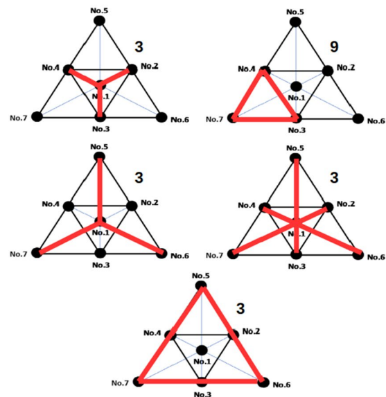
Fig. 2 Survey geometry. a Stations in the KUM-LL array (red circles). The short side is 481 m, and the long side is 962 m. b Sampling schemes of nested-triangle arrays with the different groups of interstation distances (red colors) that are binned and stacked in this ambient noise study. On the top-right of each triangular array, the number of different interstation distance pairs is shown (i.e., 3, 9, 3, 3, and 3 for the longest path)
