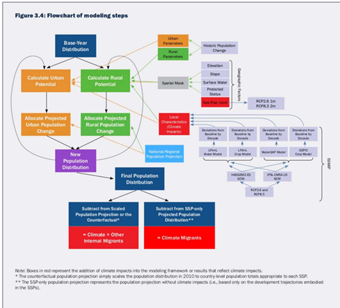
Figure 1 Schematic diagram of how climate migration is modeled in the Groundswell project (Rigaud et al. 2018: 64).
