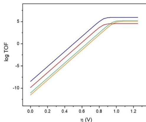
Fig. 6. Catalytic Tafel plots relating TOFs and applied overpotentials ( \eta ) for C1 (blue), C2 (orange), C3 (green), C4 (red).
