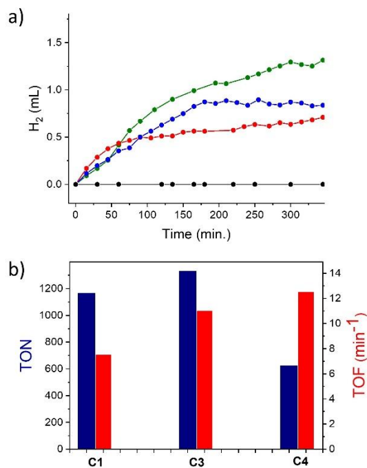
Fig. 7. a) \text{H}_2 evolution in mL over time for solutions of 5 \mu\text{M} catalysts C1 (blue) C3 (green), C4 (red) and without catalysts (black). The experiments were performed in 1.0 M acetate buffer at pH 4.0 with 0.1 M of ascorbic acid and 0.5 mM [\text{Ru}(\text{bpy})_3]\text{Cl}_2 at 20^\circ\text{C} and the solutions were irradiated with LED light at 475 nm. b) Maximum TONs and TOFs for C1 , C3 and C4 .
