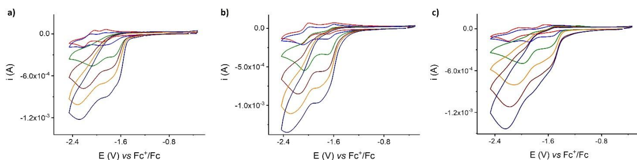
Fig. 5. Cyclic voltammograms of 1 mM of catalyst C2 (a), C3 (b) and C4 (c) recorded in CH_3CN 0.1 M of TBAPF_6 at 30 V s^{-1} with glassy carbon as working electrode and increasing amounts of TFA (0 red, 1 blue, 5 green, 10 brown, 15 orange and 20 blue navy mM).
