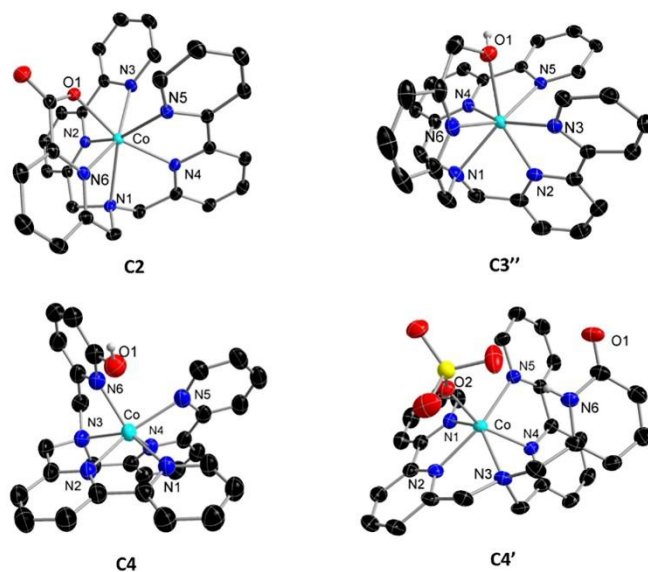
Fig. 2 Crystal structures of complexes C2 , C3'' and of the two tautomers C4 (enol form) and C4' (keto form). Colour code: Co (turquoise), N (blue), O (red), C (black), S (yellow), H (white). Non coordinating counterions (i.e., BF 4 - , PF 6 - and SO 4 2- ), solvents, and other hydrogen atoms have been omitted for clarity.
