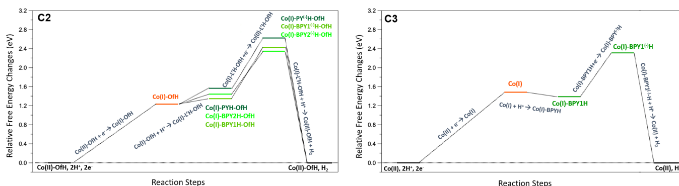
Fig. 9. Calculated free energies profiles in acetonitrile for the possible reaction steps involved in the proposed mechanism for C2 (left) and C3 (right). Values and profiles of the relative free energy changes ( \Delta G ) are given in Table ES6. The zero is defined as the free energy of the Co(II) compound (Co(II)-OfH for C2 ; Co(II) for C3 ) plus that of two protons with an activity of 1 (apparent pH = 0 in acetonitrile) and two electrons at the potential of NHE in acetonitrile. For C2 L' = BPY1, BPY2, PY. The corresponding structures can be found in Fig. ES26.
