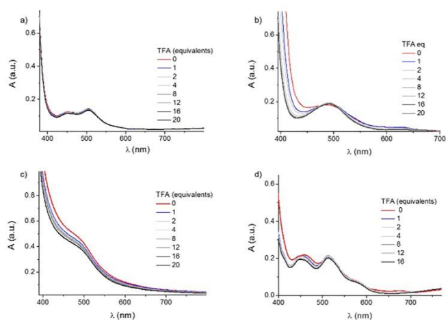
Fig. 3 UV-Vis spectra of 4 mM solutions of complex C1 (a), C2 (b), C3 (c), C4 (d) in \text{CH}_3\text{CN} at increasing amounts of TFA keeping the final volume (2 mL) unchanged.
