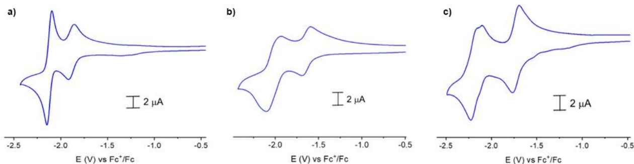
Fig. 4 Cyclic voltammograms (CVs) of 1 mM solution of complex (a: C2 , b: C3 , c: C4 ) recorded at 0.1 \text{ V s}^{-1} in \text{CH}_3\text{CN} , 0.1 M TBAPF 6 with glassy carbon as working electrode.
