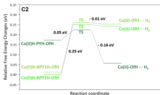
Fig. 10. Calculated free energy profiles ( \Delta G ) starting from the second protonation step until formation of H_2 , for C2 (left) and C3 (right). At this step, once formed, H_2 is still in interaction with the complex (see structures in Figure ES26). The structures corresponding to stationary points (minima and transition states, TS) are given in Figure ES26, including the imaginary frequency of the most relevant TSs.
