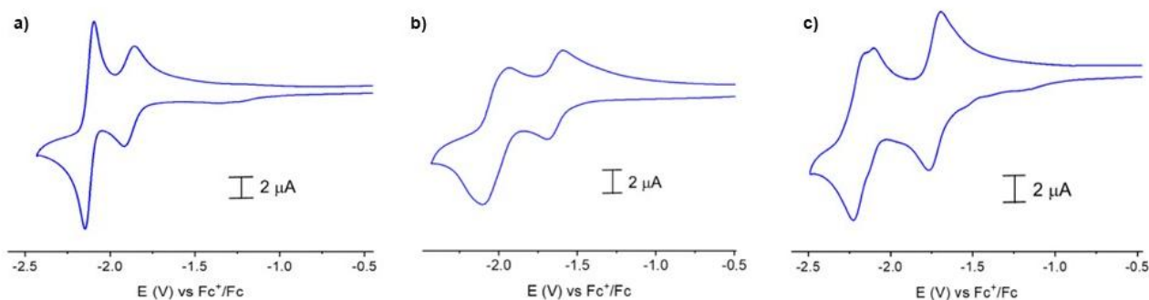
Fig. 4 Cyclic voltammograms (CVs) of 1 mM solution of complex (a: C2 , b: C3 , c: C4 ) recorded at 0.1 \text{ V s}^{-1} in \text{CH}_3\text{CN} , 0.1 M \text{TBAPF}_6 with glassy carbon as working electrode.
