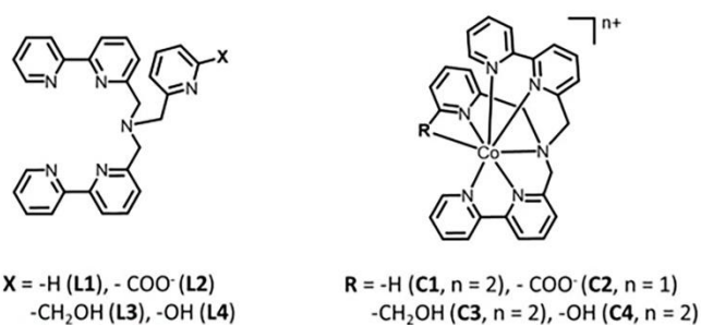
Fig. 1 Structures of the ligands L1-L4 (left) and of the corresponding Co complexes ( C1-C4 ). For sake of clarity, the description of the different counterions of complexes is provided in the text.
