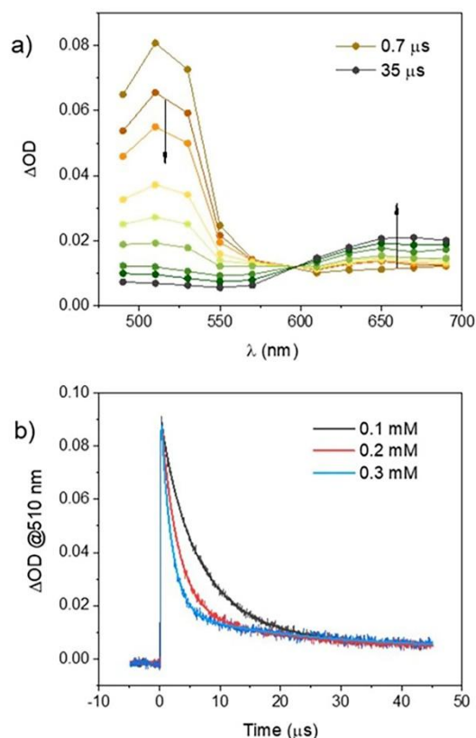
Fig. 8. a) Transient absorption spectra between 0.7–35 \mu\text{s} obtained by laser flash photolysis (excitation at 532 nm) of a solution containing 70 \mu\text{M} [\text{Ru}(\text{bpy})_3]^{2+} , 0.1 M ascorbic acid, and 0.1 mM C3 in 1 M acetate buffer; b) kinetic traces at 510 nm at 0.1–0.3 mM C3 (fitting was performed using a biexponential function in which the first component is associated to the reaction in eq. 3, the second component to the charge recombination between Co(I) and the ascorbate radical).
