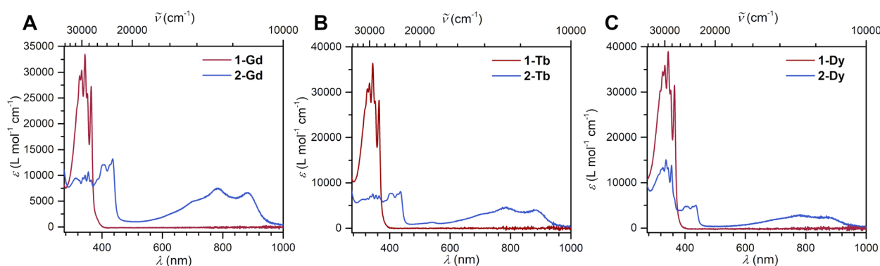
Fig. 2 Superimposed UV-vis spectra of [(Cp* 2 Ln)(μ-Bbim)] ( 1-Ln , in red), and [K(crypt-222)][(Cp* 2 Ln)(μ-Bbim)] ( 2-Ln , in blue), taken in THF. Concentrations: (A) 1-Gd : 2.636 \times 10^{-5} \text{ mol L}^{-1} , 2-Gd : 3.198 \times 10^{-5} \text{ mol L}^{-1} . (B) 1-Tb : 1.389 \times 10^{-5} \text{ mol L}^{-1} , 2-Tb : 2.307 \times 10^{-5} \text{ mol L}^{-1} . (C) 1-Dy : 1.353 \times 10^{-5} \text{ mol L}^{-1} , 2-Dy : 1.114 \times 10^{-4} \text{ mol L}^{-1} .
