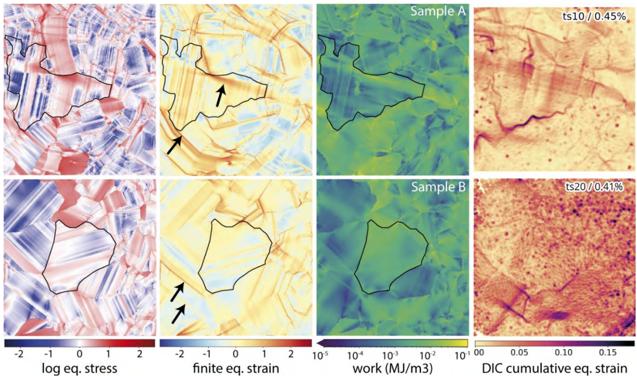
Figure 8. Full-field simulations of normalized equivalent stress, equivalent strain, and plastic work fields at a bulk longitudinal shortening of 0.5% (with compression direction vertical) alongside finite equivalent strain maps derived from DIC data at similar bulk shortenings (right-hand column). Two grains are delineated to facilitate comparison with the DIC data. The arrows on the simulated strain maps indicate sites where strain localisation is also observed in the experimental data.
