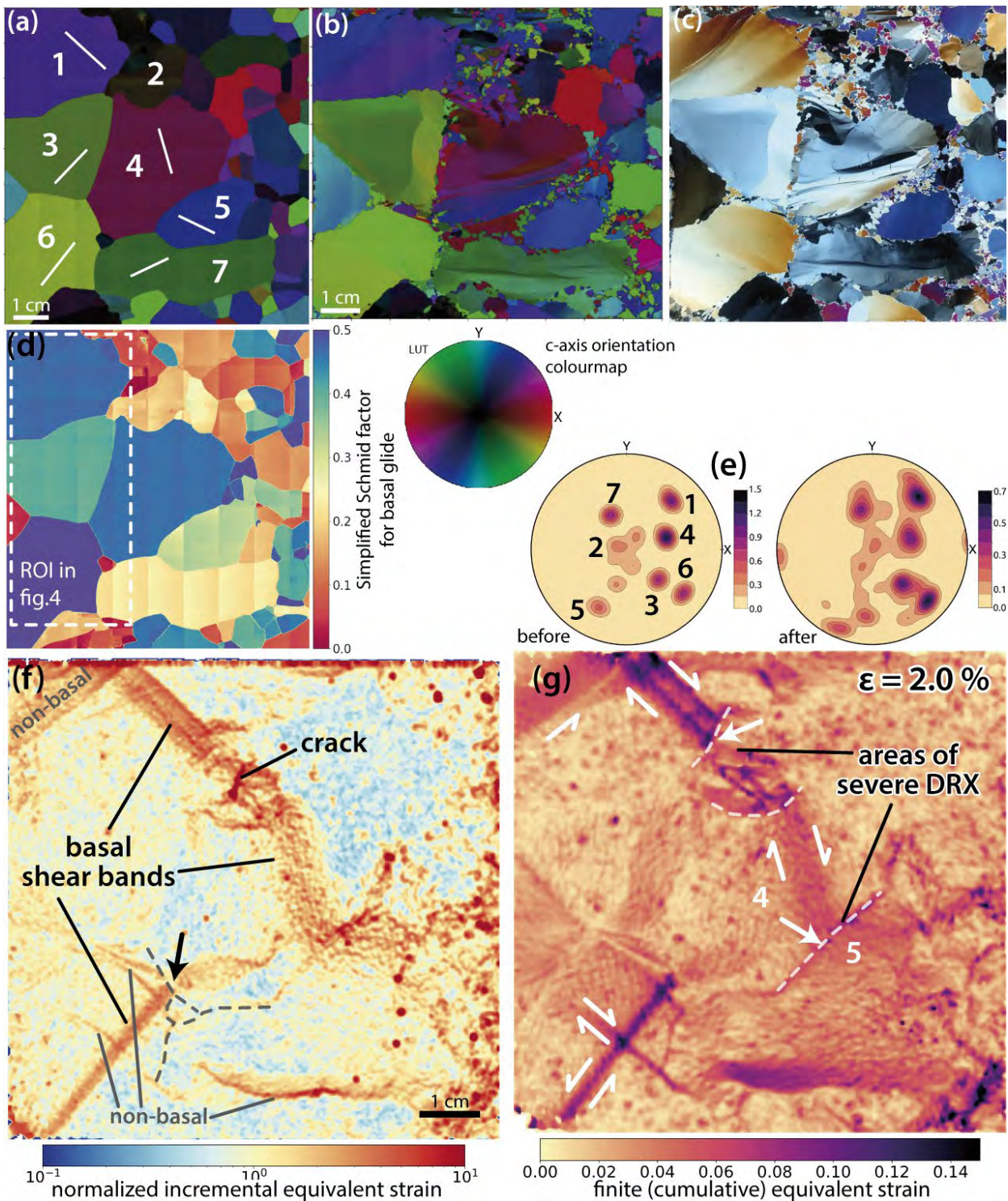
Figure 2. Microstructure, Schmid factor for basal glide, pre- and post-deformation CPO maps, and strain field at 2.0% bulk strain for sample A. The compression direction is vertical in all images. (a, b) Pre- and post-deformation (9.5% bulk shortening) c-axis orientation maps. The projection of the basal planes onto the sample surface in the numbered grains is indicated by white lines in (a). (c) Post-deformation cross-polarized light image. (d) Schmid factor map for basal glide according to initial crystal orientations. Note that grains #1, #4, #6 have high Schmid factors (c-axis at \sim 45\text{--}73^\circ to the compression normal), whereas grain #2 and #7 have moderate to low Schmid factors. The square indicates the region of interest (ROI) for which DIC could be performed until the end of the experiment (cf. figure 4). (e) Pre- and post-deformation contoured c-axis pole figures with orientations. Upper hemisphere equal-area projections. (f) Normalized incremental Von Mises (2D) equivalent strain at 2.0% of bulk strain. Basal and non-basal shear bands, the location of the crack produced at 1.4% of shortening and a few selected grain boundaries (dashed lines) are indicated. The black arrow indicates an example of slip transfer across a grain boundary (from grain #6 to #4). (g) Finite (cumulative) Von Mises 2D equivalent strain at 2.0% of bulk strain. The white dashed lines and arrows
