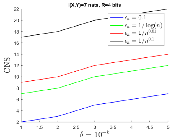
Fig. 2: Critical Number of Samples (CNS) predicted by Theorem 2 across different values of \delta = 10^{-k} . The values used are \xi(R) = 3 , I(X; Y) = 7 , R = 4 and C_X(P, Q) = 2.47 .
