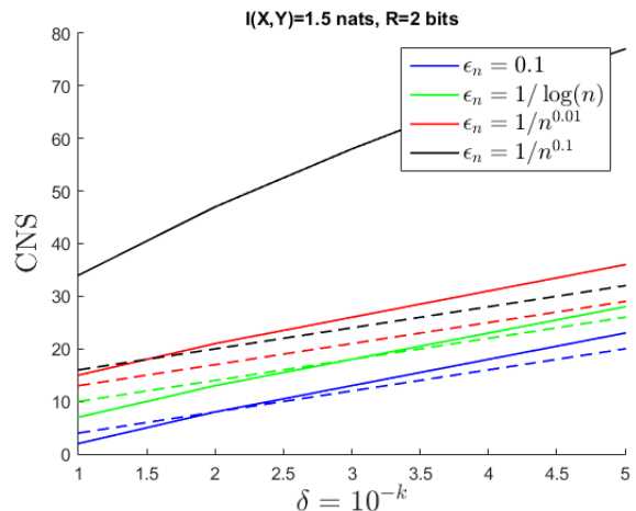
Fig. 3: CNS predicted by Th. 2 across different values of \delta = 10^{-k} . Low rate case with \xi(R) = 0.7 , I(X; Y) = 1.5 , R = 2 and C_X(P, Q) = 1.92 . The dashed lines show an estimation of the exact CNS obtained from \beta_n(\epsilon_n, R) .
