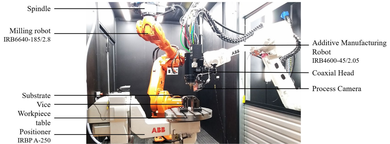
Fig. 2. Overview of the WLAM setup.
