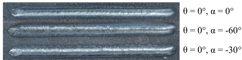
Fig. 5. Beads with or without stubbing (welding direction from right to left).
