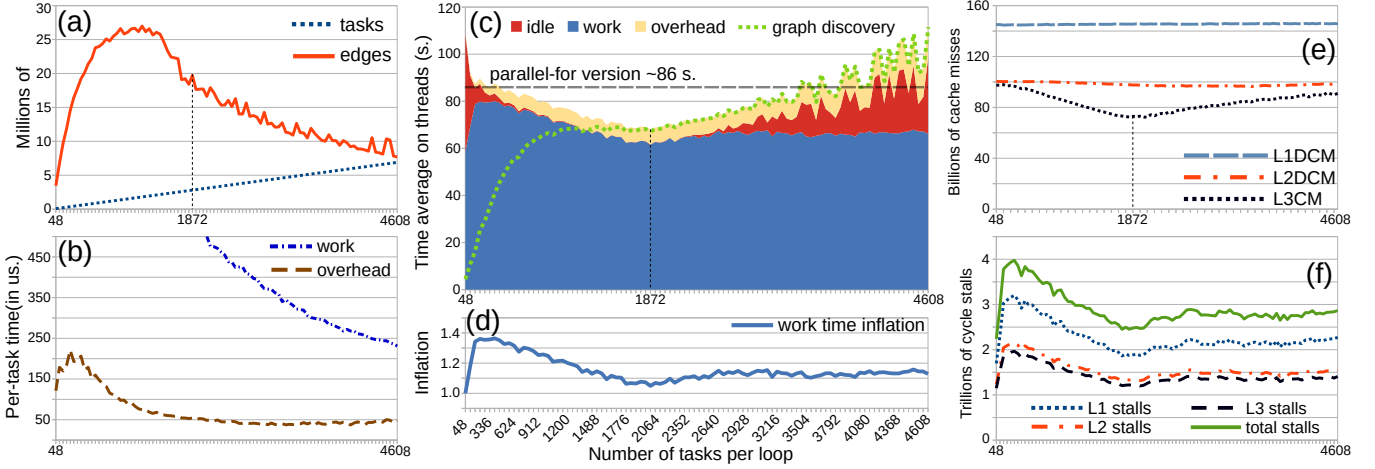
Figure 2: LULESH on a 24-cores Skylake node using MPC-OMP with -s 384 -i 16 -tel tasks-per-loop
