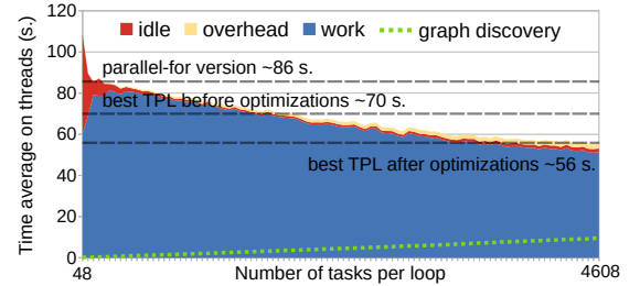
Figure 6: LULESH on Intel Skylake node with optimizations
