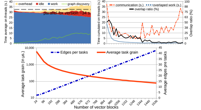
Figure 9: HPCG performances on 32 MPI processes on Intel processors for a matrix with n=41,943,040 on i=128 iterations
