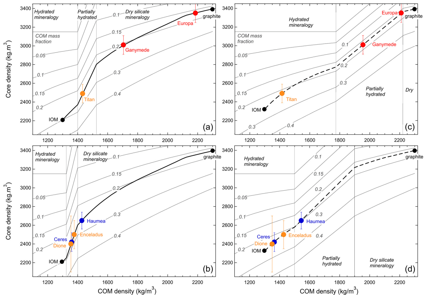
Fig. 2. Densities and proportions of COM (thick lines) inferred for (a) large bodies where pressure fixes the dehydration interval at \sim 593\text{--}853\text{ K} , and (b) small bodies where pressure fixes the dehydration interval at \sim 493\text{--}653\text{ K} . Densities of refractory core-forming mixtures (thin curves) are calculated for various mass fractions of COM and SSC in hydrated and dry core mineralogies of density \sim 3150\text{ kg/m}^3 , and \sim 3750\text{ kg/m}^3 , respectively. Evolution of the core density assumes a solar fraction of COM whose density and composition evolves as temperature increases according to pyrolysis experiments (thick curve). Decompressed densities of cores in seven bodies are reported to obtain the corresponding COM density and temperature window of metamorphism (Fig. 3). (c) and (d) same as (a) and (b) with COM density and composition calculated with the Vitrimat model (dashed thick curve). Dehydration windows are shifted to higher COM density because densification occurs at lower temperature than that inferred from pyrolysis experiments (see Fig. 3 and section 3.2). Note that differentiated cores of Ganymede and Europa with SSC density of up to 3800\text{ kg/m}^3 would increase the amount of COM by 1–2% (see section 2.1). For the sake of clarity, partially hydrated density is linearly interpolated between hydrated and dry densities. Same color code as Fig. 1.
