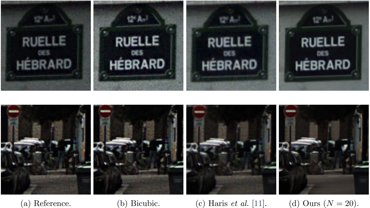
Figure 10: Comparison of different methods for \times 2 zoom on a real burst from [15]. The images are demosaiced using [10] and upscaled using several methods. Our pipeline manages to accurately recover the shape of the letters while removing the image noise. Better seen by zooming on a computer screen.
