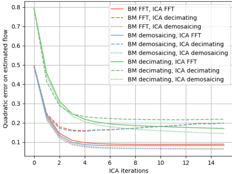
Figure 1: Comparison of the registration error for different methods. We compare the two stages of the presented alignment pipeline for three different raw-to-grayscale image conversion strategies: On the decimated quad Bayer image [13], or the full-resolution images obtained via demosaicking or FFT perfect low-pass filtering [4]. Running the two algorithms sequentially on the FFT-filtered images, with 3 ICA iterations, is the optimal strategy.
