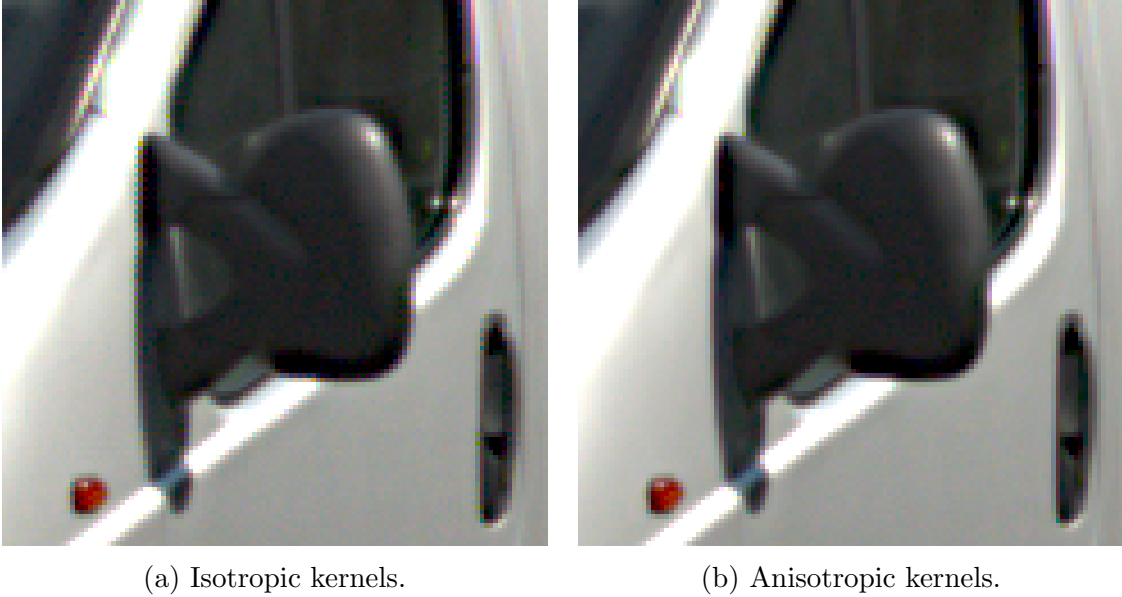
Figure 4: Example of image demosaicing illustrating the advantage of using anisotropic stretched kernels in the case of edges. Isotropic kernels with k_{shrink} = k_{stretch} = 1 in (a) cause zipper artifacts, that are less prominent when stretching kernels along edges with k_{stretch} = 4 and k_{shrink} = 2 in (b).
